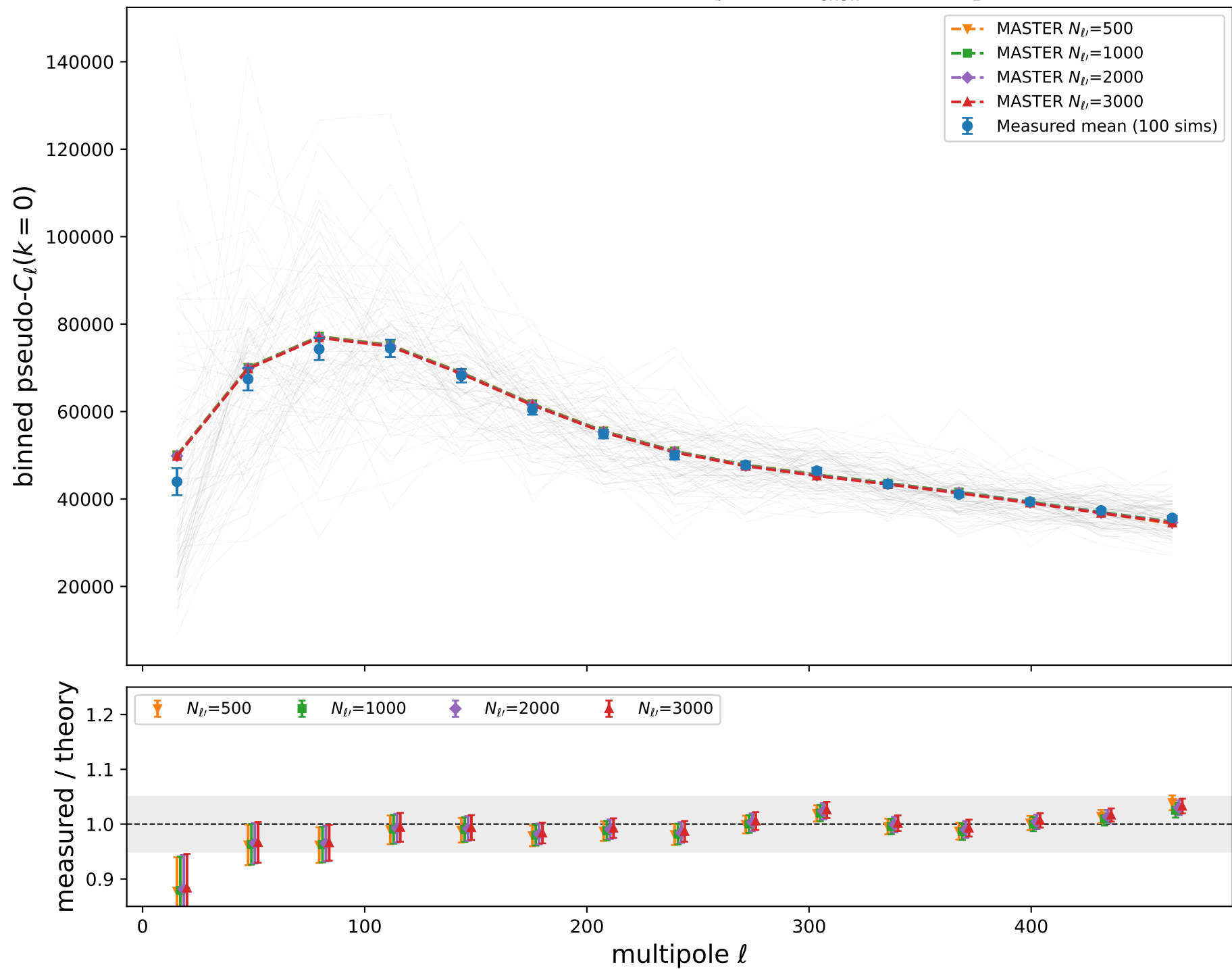
Floor-subtracted MASTER: 100 sims, N_{\ell}=500 , N_{\text{skew}}=9600 , b_1=-0.1521
