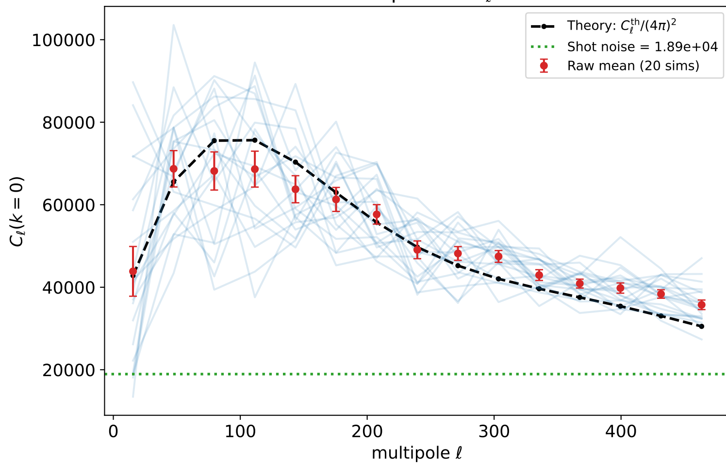
Raw pseudo- C_\ell
