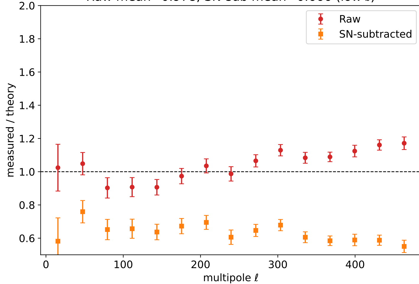
Raw mean=0.978, SN-sub mean=0.666 (low \ell )
