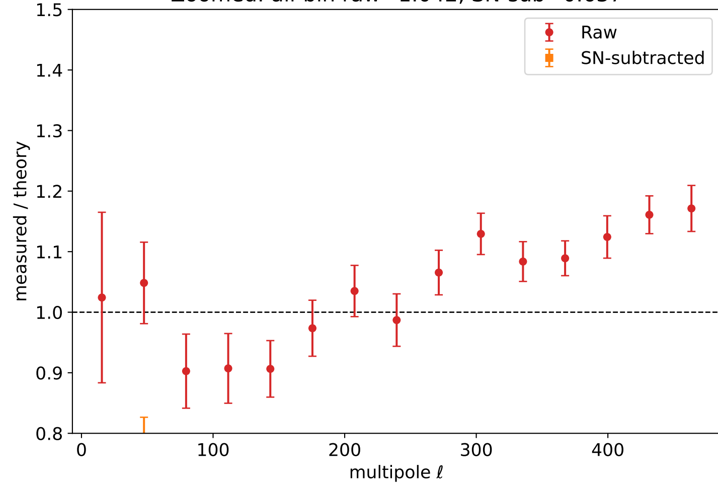
Zoomed: all-bin raw=1.042, SN-sub=0.637
