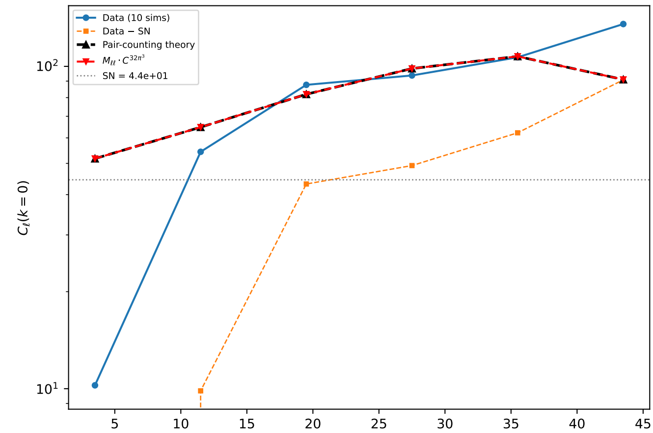
\chi_{shift} = 5000 , patch= 14^\circ , Nskew=4096
