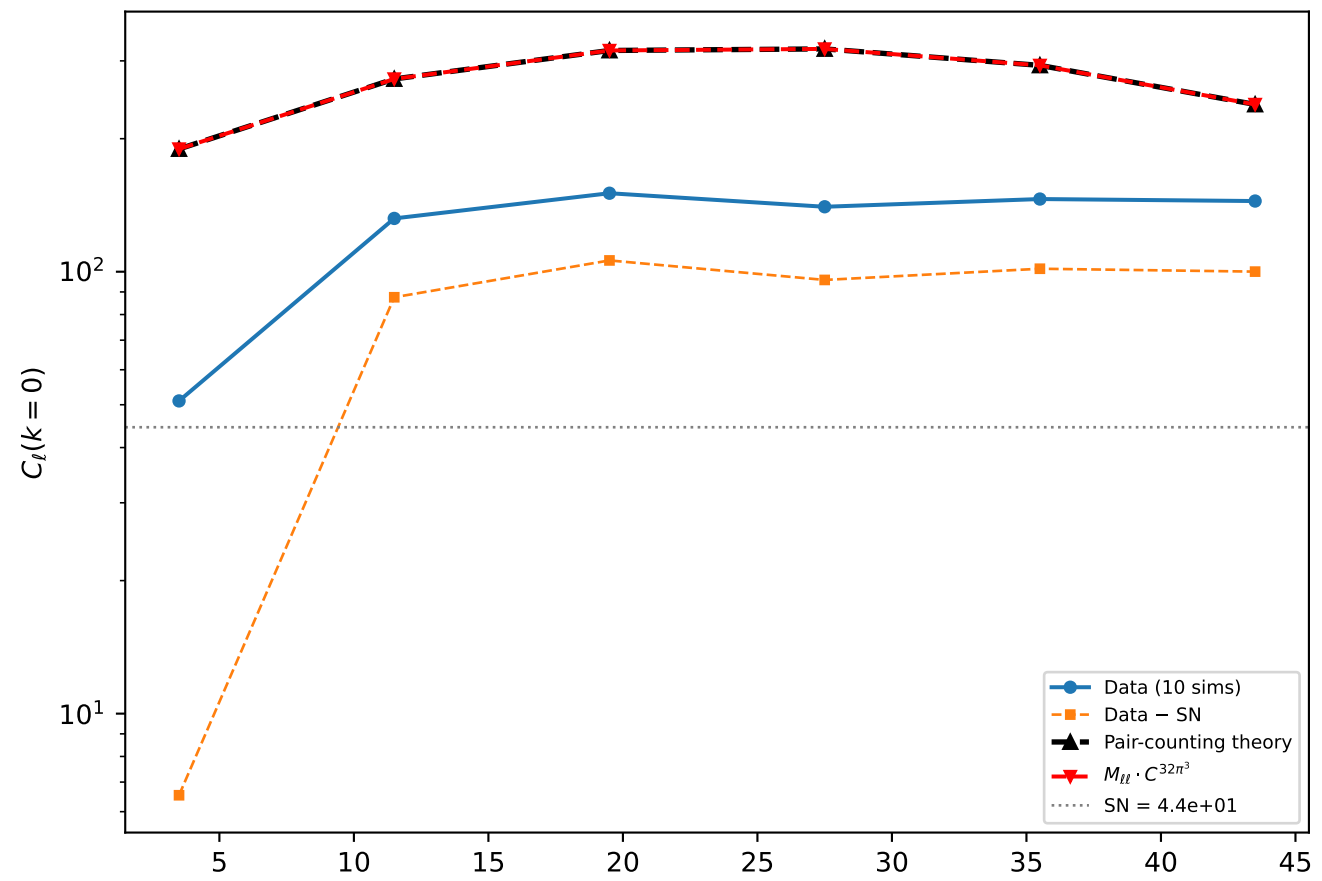
\chi_{shift} = 800 , patch= 53^\circ , Nskew=4096
