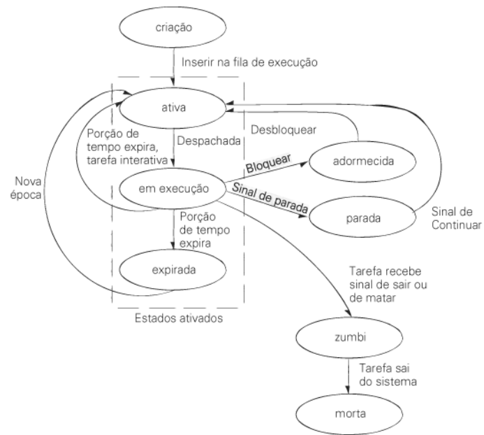
Figura 3.10: Thread Status
