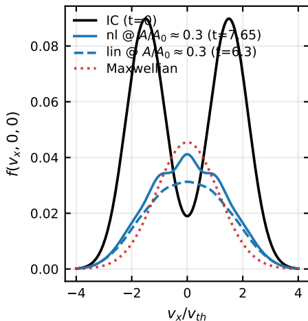
(c) 1 species (sp) vx-slice
