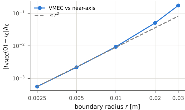
(a) on-axis rotational transform
