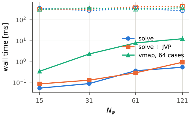
(a) warm (solid) vs compile + first call (dotted)
