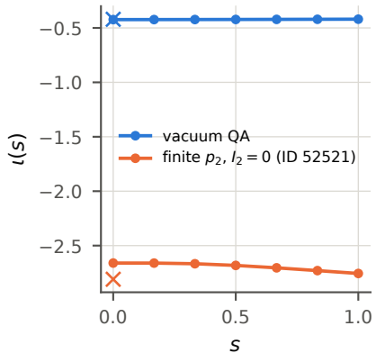
(a) \iota (x: near-axis \iota_0 )
