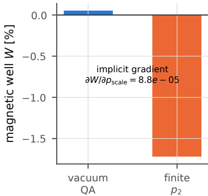
(c) magnetic well
