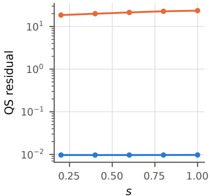
(b) quasisymmetry error
