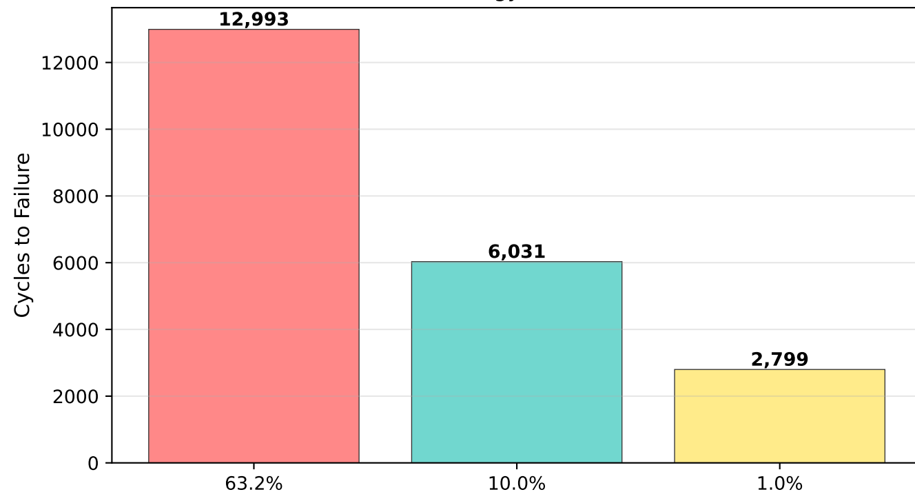
Fatigue Life at Different Failure Percentiles Strain Energy: 0.6542 MPa
