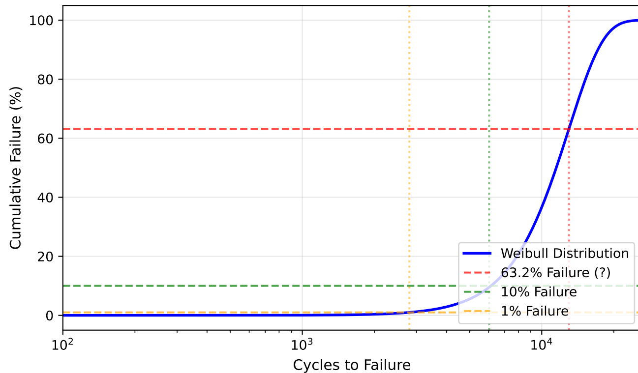
Weibull Distribution - SAC305 \beta=3.00 , \eta=12,993
