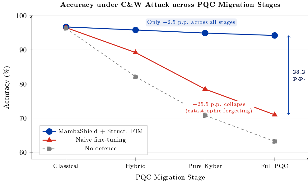
Figure 4.8 – Accuracy under C&W attack across four PQC migration stages (Classical \rightarrow Hybrid \rightarrow Pure Kyber \rightarrow Full PQC). MambaShield with structured FIM maintains accuracy within 2.5 p.p. across all stages, while naive fine-tuning collapses by 25.5 p.p. due to catastrophic forgetting of classical traffic patterns.
