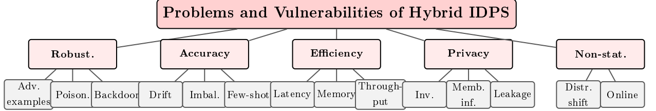
Figure 1.4 – Systematisation of problems and vulnerabilities motivating the development of Models M1–M7. Each of the five axes is covered by one or several developed models (direct mapping is given in Table 1.1 after the analysis of existing limitations).
