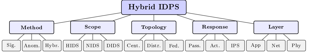
Figure 1.1 – Hierarchical classification of Hybrid IDPS along five orthogonal axes. By detection method — signature-based (deterministic lookup against a database of known patterns), anomaly-based (statistical or learned deviation from a normal profile), and hybrid (combination of both). By scope — host-based (HIDS), network-based (NIDS), and distributed (DIDS). By deployment topology — centralised, distributed, federated. By response character — passive (alerting only), active (in-line intervention), and IPS (full blocking). By stack layer — application, network, and physical.
