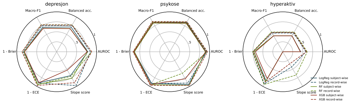
Figure 6: Multi-metric profile of the models per cohort (AUROC, balanced accuracy, macro-F1, 1 - \text{Brier} , 1 - \text{ECE} and a slope score 1 - |1 - \text{slope}| ) under subject-wise (solid) and record-wise (dashed) cross-validation. Leakage expands every axis at once; on HYPERAKTIV the honest profile collapses to chance while the leaky profile does not.
