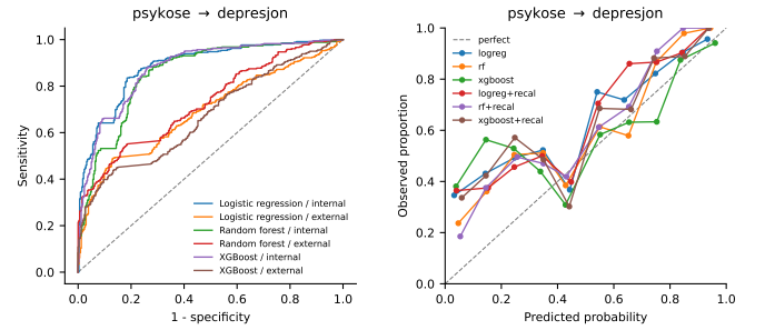
Fig. 3. PSYKOSE→DEPRESJON. Left: ROC of internal (subject-wise CV on PSYKOSE) and external (frozen model on DEPRESJON) predictions. Right: reliability of the external predictions before and after recalibration fitted on the training cohort.
