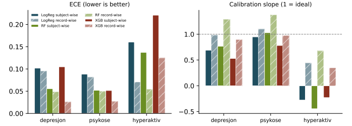
Fig. 4. ECE (left) and calibration slope (right) under subject-wise (solid) and record-wise (hatched) cross-validation.
