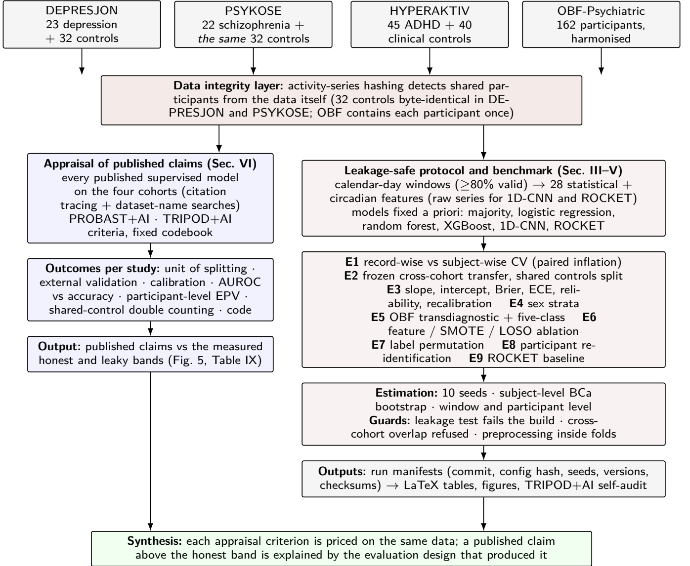
Fig. 1. Architecture of the study. Four open actigraphy cohorts pass through a data-level integrity check (participant hashing) into the leakage-safe protocol and benchmark (Sections III to V) and the appraisal of published claims (Section VI); the synthesis maps every appraisal criterion to a measured cost.
