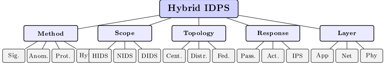
Figure 1.1 – Hierarchical classification of Hybrid IDPS along five orthogonal axes. By detection method — signature-based (deterministic lookup against a database of known patterns), anomaly-based (statistical or learned deviation from a normal profile), protocol-analysis-based (context-aware analysis of the correctness of network, application, and industrial protocols and their states), and hybrid (combination of the three preceding, augmented with the learnable Models M1–M7). By scope — host-based (HIDS), network-based (NIDS), and distributed (DIDS). By deployment topology — centralised, distributed, federated. By response character — passive (alerting only), active (in-line intervention), and IPS (full blocking). By stack layer — application, network, and physical.
