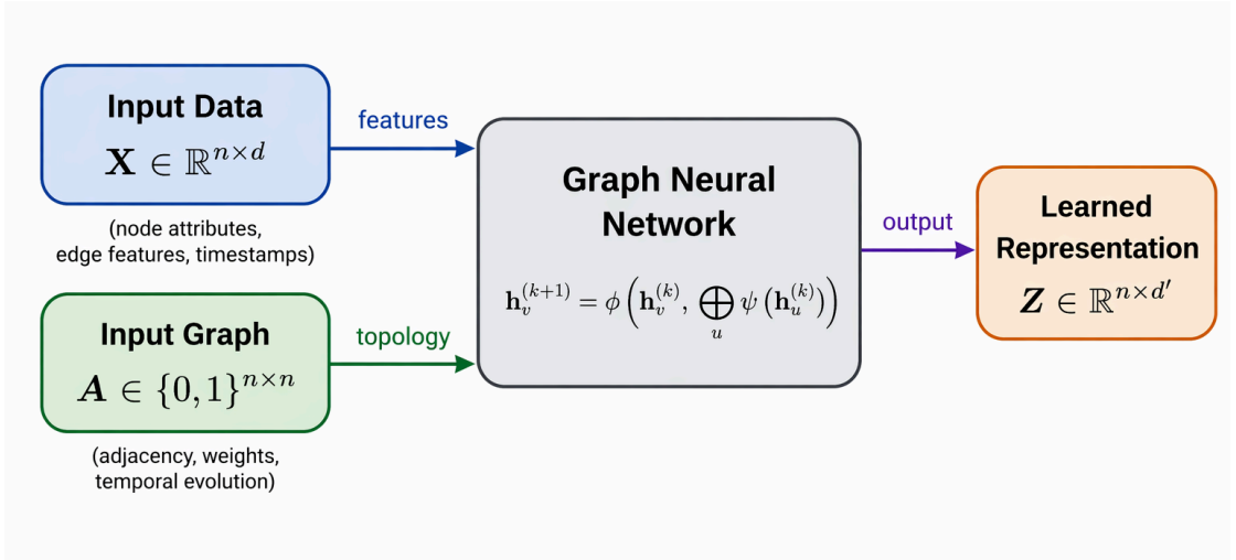
Figure 1 – Dual-input nature of the GNN-based detectors that constitute one branch of the learnable models used in Hybrid IDPS. The network receives both numerical data (feature matrix \mathbf{X} ) and relational structure (adjacency matrix \mathbf{A} ) as inputs. Perturbation of either input can compromise the learned representation, motivating the framework for improving the robustness and efficiency of Hybrid IDPS developed in this dissertation.
