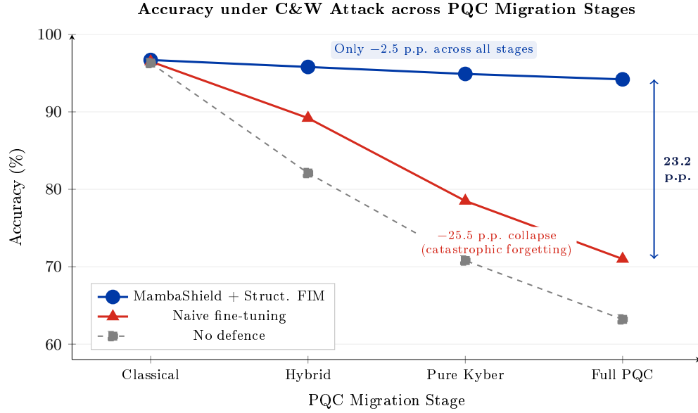
Figure 4.4 – Accuracy under C&W attack across four PQC migration stages (Classical \rightarrow Hybrid \rightarrow Pure Kyber \rightarrow Full PQC). MambaShield with structured FIM maintains accuracy within 2.5 p.p. across all stages, while naive fine-tuning collapses by 25.5 p.p. due to catastrophic forgetting of classical traffic patterns.
