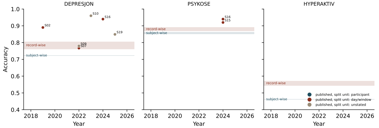
Figure 2: Published best accuracies (points, labelled by study ID in Table ??, coloured by the unit of splitting) against the window-level accuracy bands measured in Part II under subject-wise and record-wise five-fold cross-validation (shaded; range over logistic regression, random forest and XGBoost). The vertical axis is classification accuracy for both. Studies that report a metric other than accuracy, or no numeric value in the available text, are not plotted; all are listed in Table ??.
