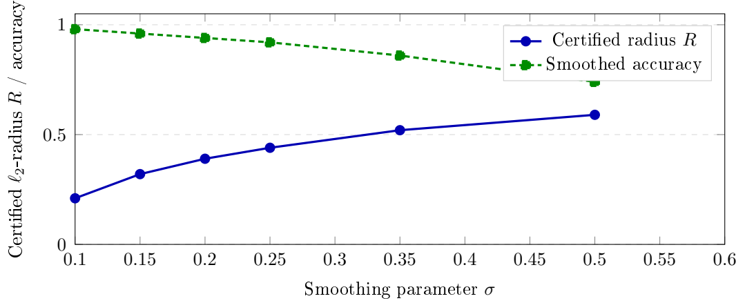
Figure 6.5 – Trade-off between the smoothing parameter \sigma , the certified \ell_2 -radius and the accuracy of the smoothed classifier (Cohen-style, \alpha = 10^{-3} ).
