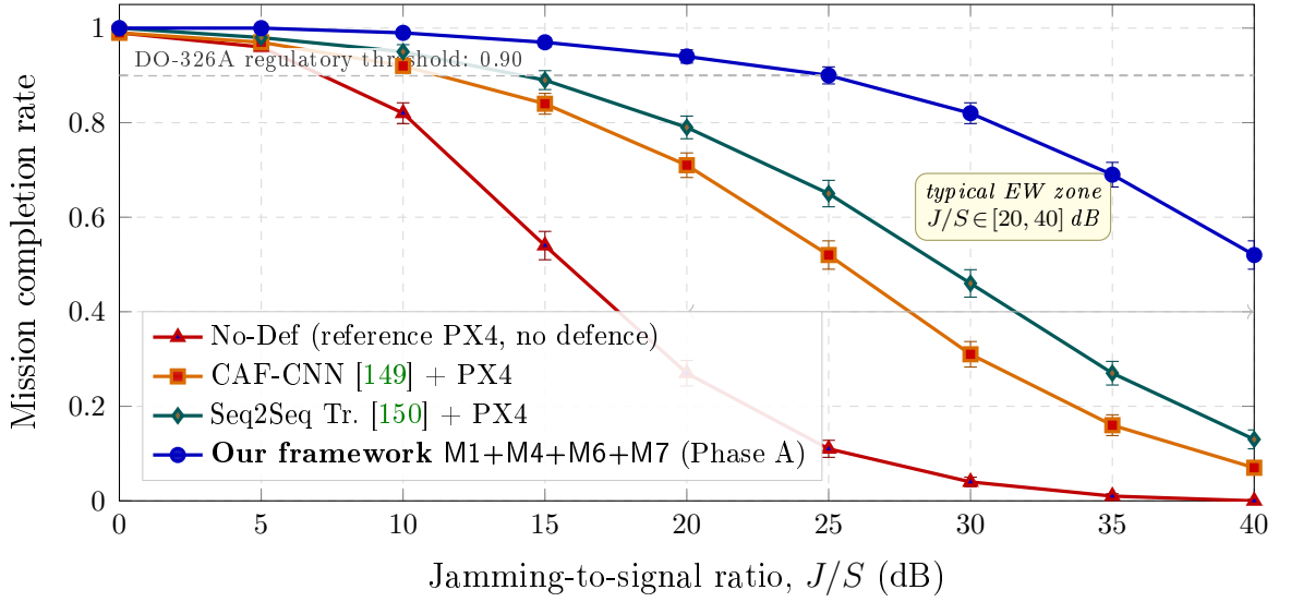
Figure 6.6 – UAV mission completion rate as a function of EW jamming intensity, measured by the jamming-to-signal power ratio ( J/S , dB). UAV-EW-Bench-2026: 5 000 simulated flights (AirSim / PX4 SITL), three mission types, three GNSS receiver models, combined adversarial loop. Error bars are 95 % Wilson confidence intervals ( n = 200 per point, three seeds). The proposed framework M1+M4+M6+M7 keeps completion above the DO-326A 0.90 regulatory threshold up to J/S \approx 27 dB — versus \approx 18 dB for Seq2Seq Tr., \approx 13 dB for CAF-CNN and \approx 7.5 dB for the unprotected PX4 reference, i.e. a 9–19 dB margin gain on the operationally meaningful metric.
