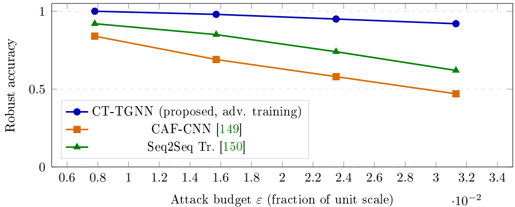
Figure 6.4 – Robust accuracy versus PGD attack budget \varepsilon for three architectures. The proposed CT-TGNN sustains robust accuracy \geq 0.92 across the entire studied range.
