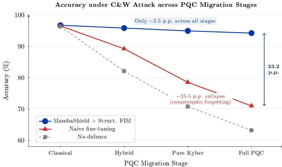
Figure 4.9 – Accuracy under C&W attack across four PQC migration stages (Classical → Hybrid → Pure Kyber → Full PQC). MambaShield with structured FIM maintains accuracy within 2.5 p.p. across all stages, while naive fine-tuning collapses by 25.5 p.p. due to catastrophic forgetting of classical traffic patterns.
