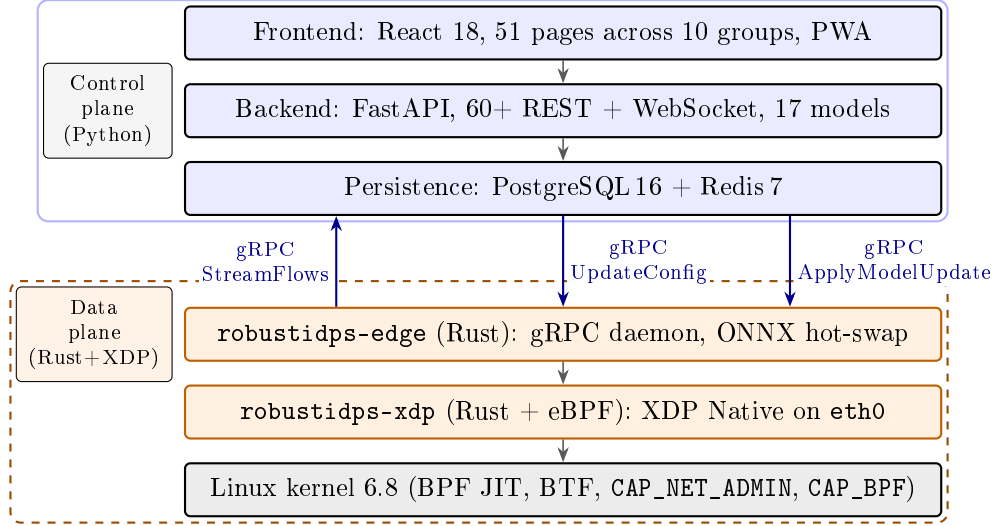
Figure 5.3 – Two-plane architecture of RobustDPS.ai v4: the Python control plane (blue frame, top) and the Rust data plane (orange dashed frame, bottom) are separated by a clean boundary and bridged by three gRPC primitives. StreamFlows — flow records streamed from the data plane to the control plane; UpdateConfig — block-list push in the reverse direction; ApplyModelUpdate — atomic delivery of the INT8 ONNX student model to running agents without service restart.
