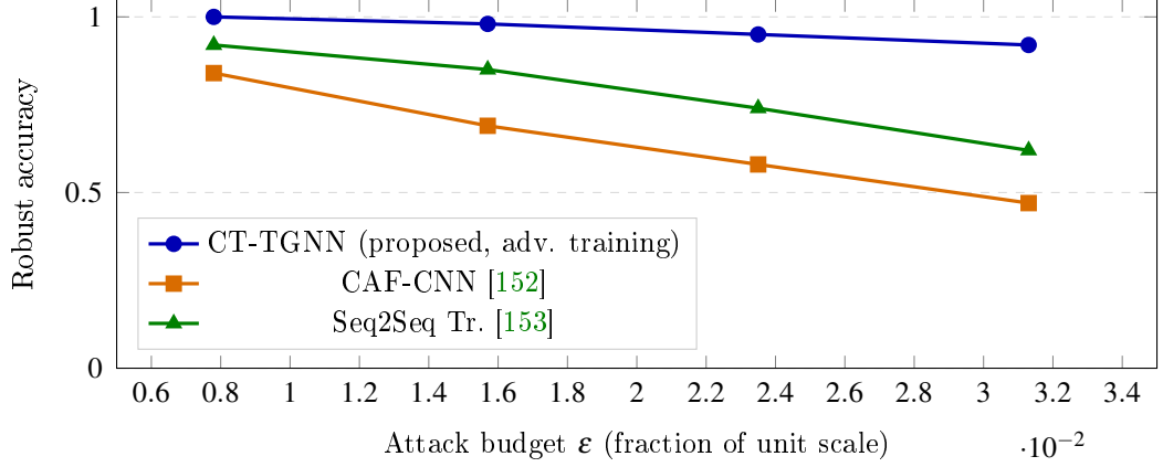
Figure 6.5 – Robust accuracy versus PGD attack budget \epsilon for three architectures. The proposed CT-TGNN sustains robust accuracy \geq 0.92 across the entire studied range.
