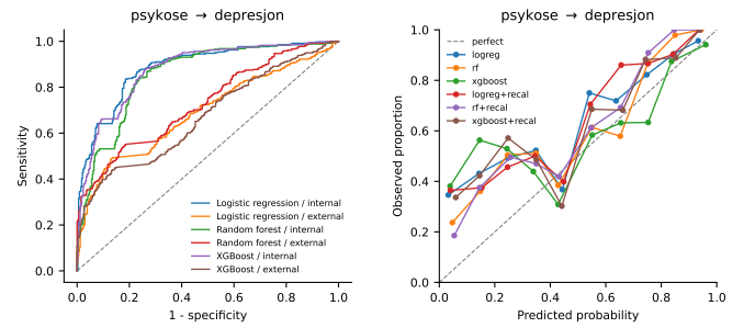
Fig. 3. PSYKOSE→DEPESJON. Left: ROC of internal (subject-wise CV on PSYKOSE) and external (frozen model on DEPESJON) predictions. Right: reliability of the external predictions before and after recalibration fitted on the training cohort.
