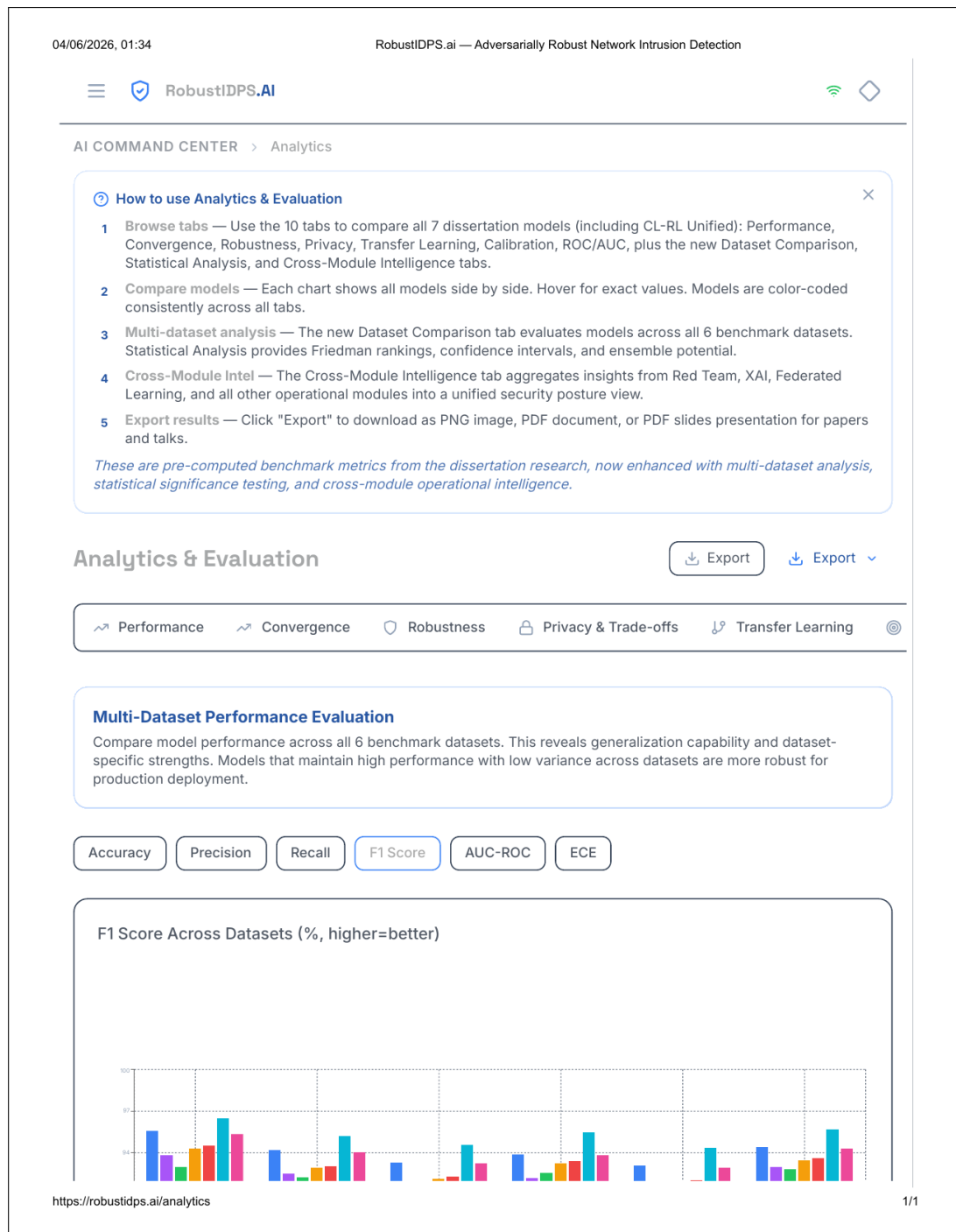
Figure 3.9 – The Analytics & Evaluation page with the “How to use” hint open: interactive explanations of the ten comparative model-evaluation tabs, with PNG/PDF export and a PDF presentation export.
