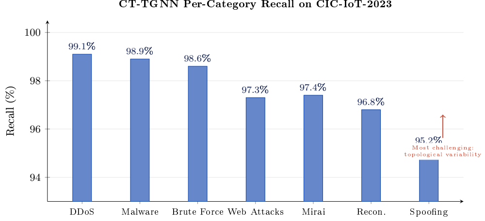
Figure 3.12 – CT-TGNN per-category recall on CIC-IoT-2023 across seven major attack families. DDoS achieves the highest recall (99.1%) while spoofing is most challenging (95.2%), reflecting the latter’s greater topological variability.
