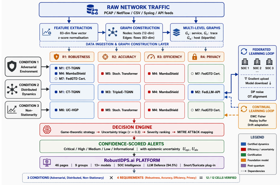
Figure 3.10 – Integrated detection pipeline showing the data flow from raw network traffic through all seven methods to severity-ranked, confidence-scored alerts. The FedLLM-API module synchronises models across boundaries under differential privacy.
