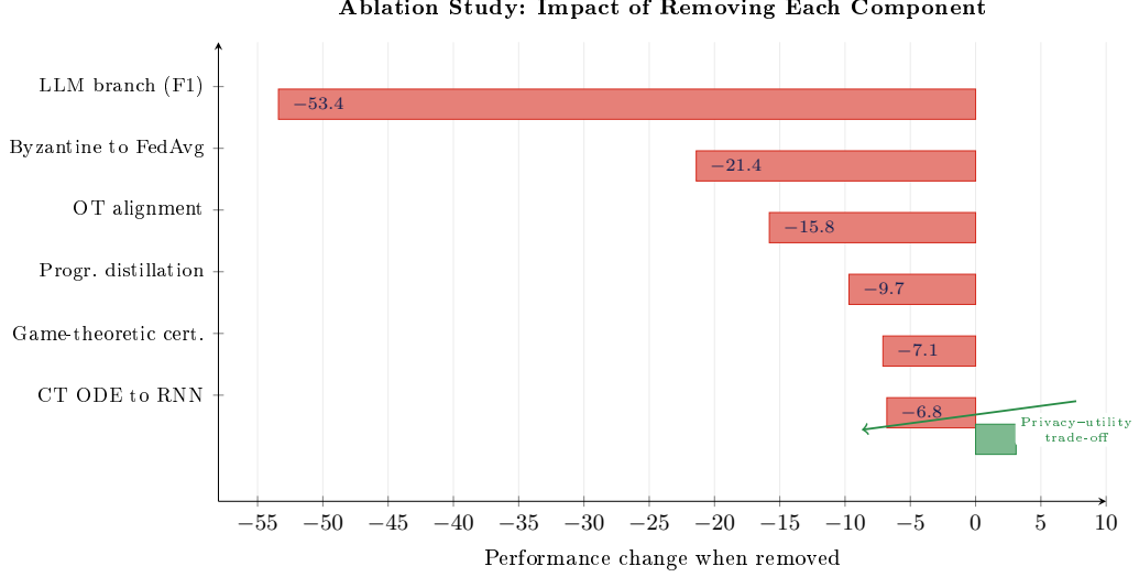
Figure 3.15 – Ablation study: performance drop when each component is removed. Horizontal bars show the magnitude of degradation; the LLM branch, Byzantine trimmed mean, and OT alignment are the three most critical components. DP noise is the only component whose removal improves accuracy (+3.1%), reflecting the privacy–utility trade-off.
