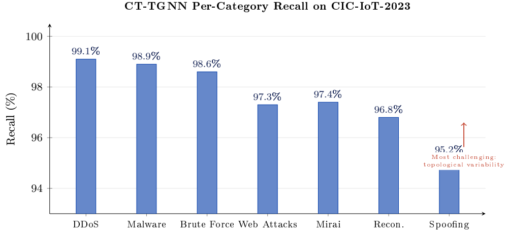
Figure 3.13 – CT-TGNN per-category recall on CIC-IoT-2023 across seven major attack families. DDoS achieves the highest recall (99.1%) while spoofing is most challenging (95.2%), reflecting the latter’s greater topological variability.
