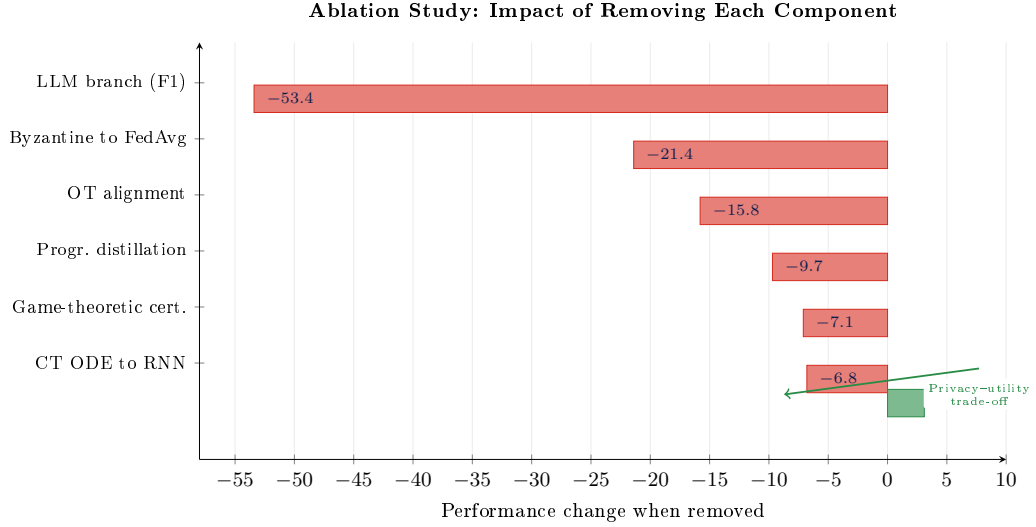
Figure 3.16 – Ablation study: performance drop when each component is removed. Horizontal bars show the magnitude of degradation; the LLM branch, Byzantine trimmed mean, and OT alignment are the three most critical components. DP noise is the only component whose removal improves accuracy (+3.1%), reflecting the privacy–utility trade-off.
