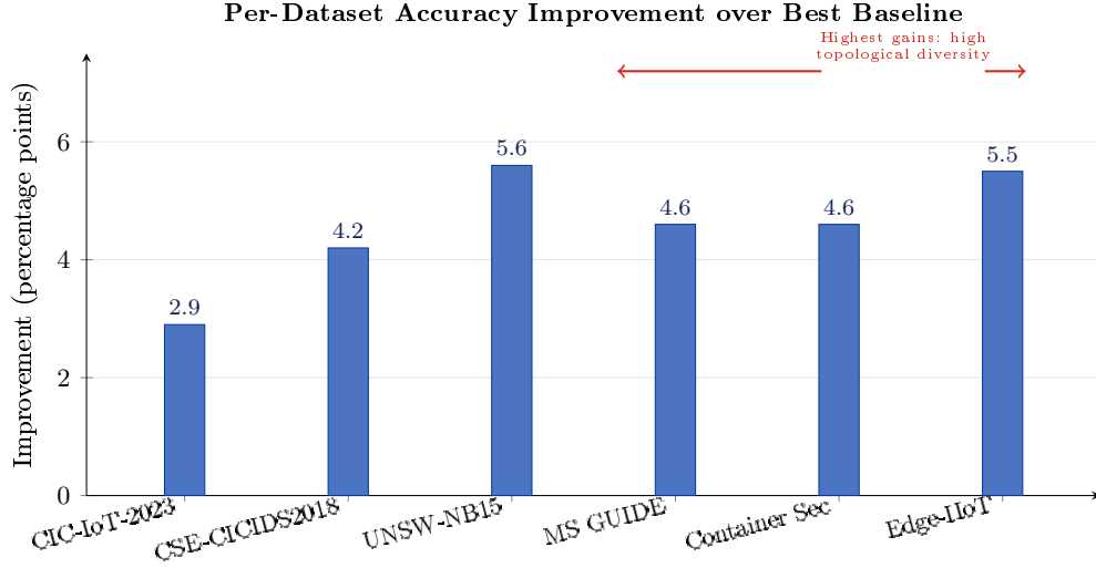
Figure 3.12 – Per-dataset accuracy improvement (percentage points) of the unified framework over the best single baseline. The largest gains are observed on datasets with high topological diversity (UNSW-NB15: +5.6, Edge-IIoT: +5.5).
