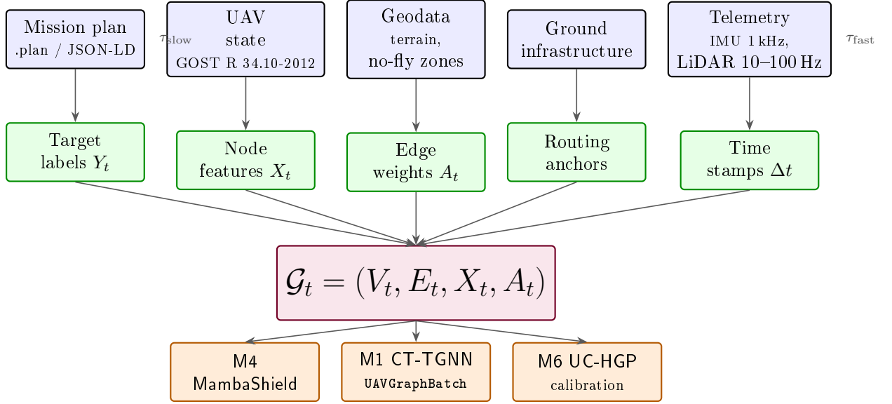
Figure 6.4 – Six-stage pipeline that converts UAV telemetry into the continuous-time dynamic graph \mathcal{G}_t and forwards it to the defensive-layer methods M1/M4/M6. Five heterogeneous sources (blue band) are processed into target labels, node features, edge weights, routing anchors and time stamps (green band), aggregated into a single graph \mathcal{G}_t (purple central node), and consumed by the defence methods (orange band) through the unified UAVGraphBatch interface. The multi-scale time constants \tau_{\text{fast}} (IMU/LiDAR) and \tau_{\text{slow}} (mission plans) absorb the heterogeneity of sensor rates.
