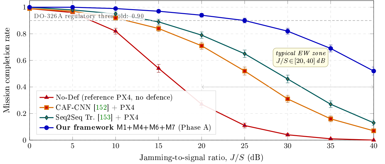
Figure 6.7 – UAV mission completion rate as a function of EW jamming intensity, measured by the jamming-to-signal power ratio ( J/S , dB). UAV-EW-Bench-2026: 5000 simulated flights (Air-Sim / PX4 SITL), three mission types, three GNSS receiver models, combined adversarial loop. Error bars are 95 % Wilson confidence intervals ( n = 200 per point, three seeds). The proposed framework M1+M4+M6+M7 keeps completion above the DO-326A 0.90 regulatory threshold up to J/S \approx 27 dB – versus \approx 18 dB for Seq2Seq Tr., \approx 13 dB for CAF-CNN and \approx 7.5 dB for the unprotected PX4 reference, i.e. a 9–19 dB margin gain on the operationally meaningful metric.
