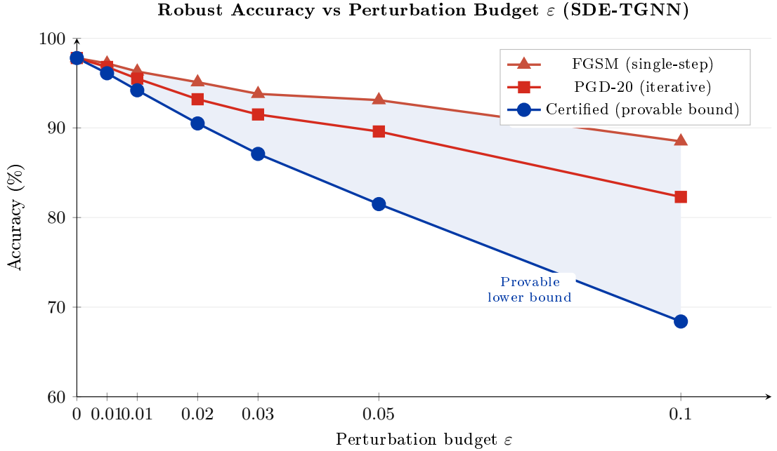
Figure 4.6 – Robust accuracy as a function of perturbation budget \varepsilon for FGSM, PGD-20, and certified (randomised smoothing) evaluations on SDE-TGNN. The certified curve provides a provable lower bound; FGSM and PGD represent empirical upper bounds under specific attack strategies.
