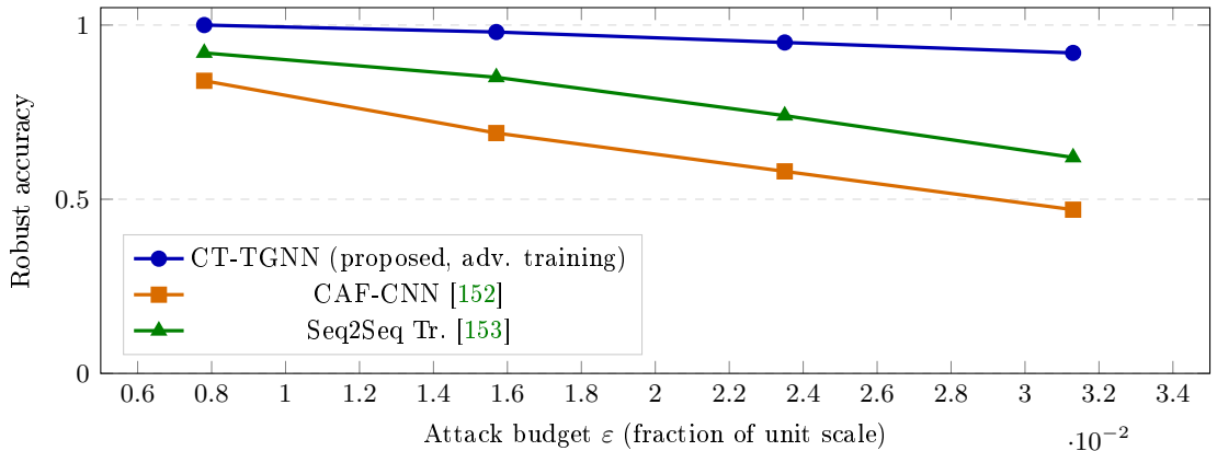
Figure 6.5 – Robust accuracy versus PGD attack budget \varepsilon for three architectures. The proposed CT-TGNN sustains robust accuracy \geq 0.92 across the entire studied range.
