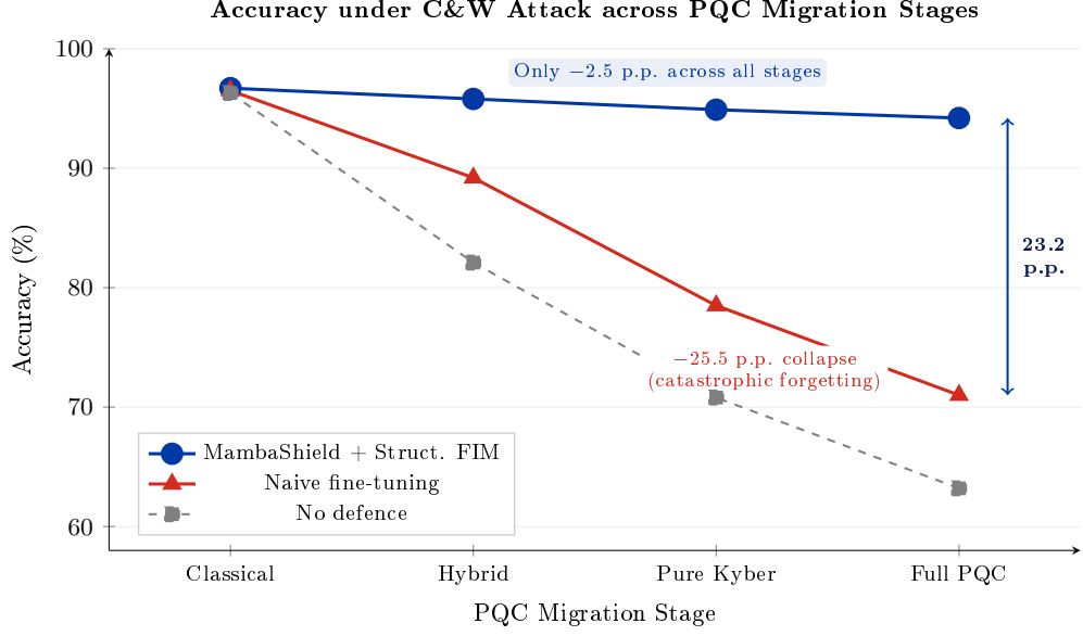
Figure 4.4 – Accuracy under C&W attack across four PQC migration stages (Classical \rightarrow Hybrid \rightarrow Pure Kyber \rightarrow Full PQC). MambaShield with structured FIM maintains accuracy within 2.5 p.p. across all stages, while naive fine-tuning collapses by 25.5 p.p. due to catastrophic forgetting of classical traffic patterns.
