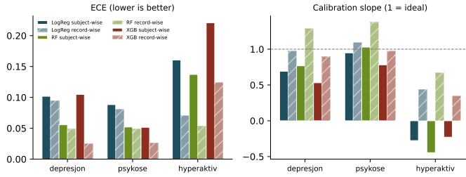
Fig. 4. ECE (left) and calibration slope (right) under subject-wise (solid) and record-wise (hatched) cross-validation.
