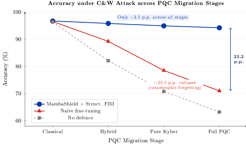
Figure 4.9 – Accuracy under C&W attack across four PQC migration stages (Classical \rightarrow Hybrid \rightarrow Pure Kyber \rightarrow Full PQC). MambaShield with structured FIM maintains accuracy within 2.5 p.p. across all stages, while naive fine-tuning collapses by 25.5 p.p. due to catastrophic forgetting of classical traffic patterns.
