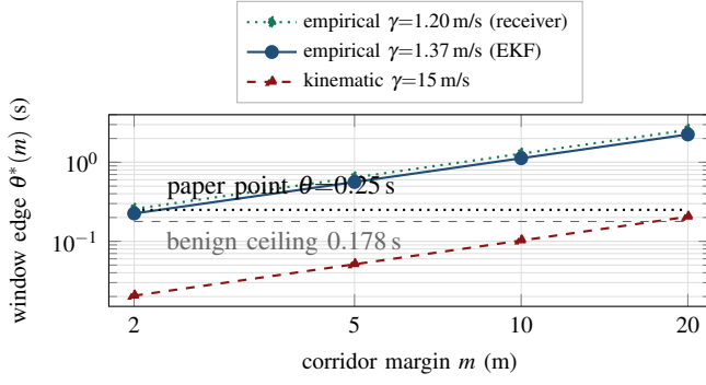
Fig. 8: The decisive sensitivity: the loosest detector setting \theta^*(m) = m/(\gamma e^{LT_c} H) whose worst-case evading tube still fits a corridor of margin m , per interface mapping. A mapping certifies the paper operating point iff its curve lies above the \theta=0.25 s line; the feasible region is bounded below by the measured benign residual ceiling (0.178 s, the FPR=0 floor). The measured rates clear the requirement \gamma_{\text{req}}=6.14 m/s at m=10 m by \sim 4.5\times ; the kinematic worst case fails at every margin.
