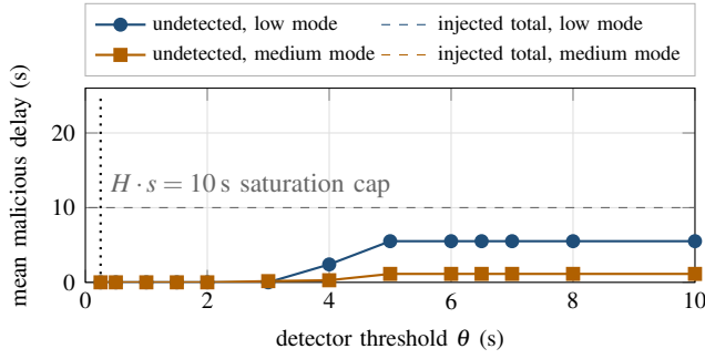
Fig. 6: The measured residual budget behind Lemma 1 (scenario 1, mean over 8 seeds \times 4 policies). The undetected delay an evader slips past the detector (solid) saturates well below the total injected delay (dashed): beyond the contact-window slack the extra delay produces missed windows flagged at any \theta , so the curve the certificate consumes flattens rather than growing.
