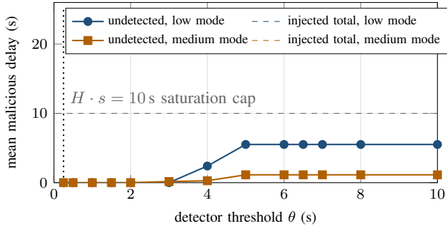
Fig. 4. The measured residual budget behind Lemma 1 (scenario 1, mean over 8 seeds \times 4 policies). The undetected delay an evader slips past the detector (solid) saturates well below the total injected delay (dashed); beyond the contact-window slack the extra delay produces missed windows that are flagged at any \theta , so the curve the certificate consumes flattens rather than growing. This is the empirical face of the \Delta(\theta) \leq H \min(\theta, s) cap.
