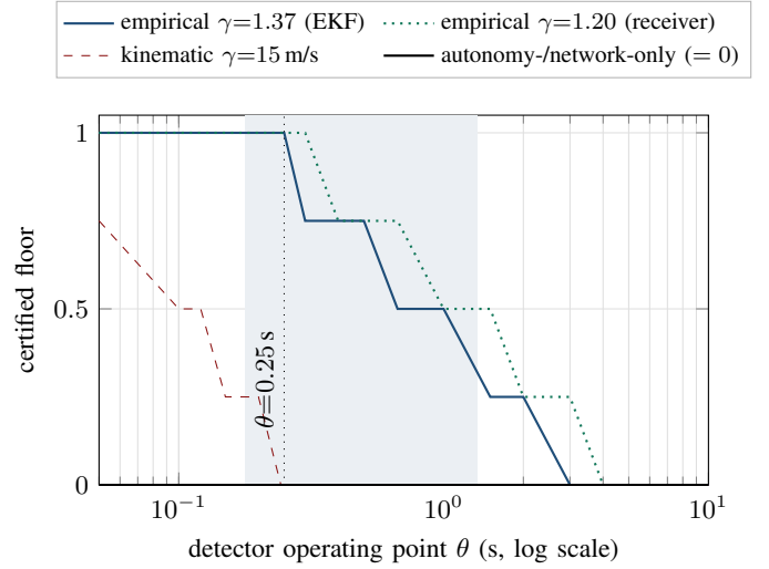
Fig. 2. The headline result, corrected. Certified floor vs. detector operating point \theta for the time-delay class (scenario 1, Grönwall tube at the measured local L=1.181 , H=2 malicious hops, corridor-margin family \{2, 5, 10, 20\} m). The result is parametric in the \theta \mapsto \delta mapping : under the kinematic worst case (red) \theta=0.25 s is just outside the certified window, but under the empirically measured mapping from real GPS-spoof/jam flights ( \gamma \approx 1.2\text{--}1.4 m/s; blue/green) \theta=0.25 s is inside at every margin (shaded: the EKF window [0.178, 1.334] s at m=10 m). Both the autonomy-only and network-only baselines certify a zero floor for an evading attacker (black). The composed guarantee is the only configuration with a nonzero certified floor. Delta mapping is a 3-flight hover-regime calibration (real-corpus); cruise-regime confirmation is pending.
