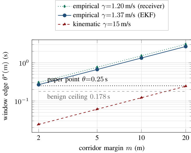
Fig. 3. The decisive sensitivity: the loosest detector setting \theta^*(m) = m/(\gamma e^{LT} H) whose worst-case evading tube still fits a corridor of margin m , per \theta \mapsto \delta mapping. A mapping certifies the paper operating point iff its curve lies above the \theta=0.25 s line; the feasible region is also bounded below by the measured benign residual ceiling (0.178 s, the FPR=0 floor). The empirically measured rates ( \gamma=1.20/1.37 m/s, receiver/EKF—an explicit error-source switch, both reported) clear the requirement \gamma_{\text{req}}=7.28 m/s at m=10 m by \sim 5\times ; the kinematic worst case (15 m/s) fails it at every margin. Real-corpus \gamma from a 3-flight hover sample; cruise regime pending.
