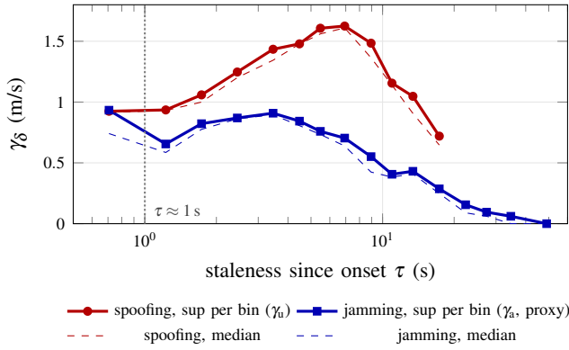
Fig. 2. The sensing side of the budget, measured on the real PX4 flights (EKF signal, baseline-corrected rate \gamma_\delta of Eq. (3)). In the first second of staleness the spoofed and the jammed estimator degrade at the same rate: the spoofer has not yet walked the fix away from where an honest estimator would put it. Beyond that, the spoofer out-runs the jammed (degraded but honest) estimator by up to 1.74\times . Authentication can buy at most the gap between the curves. The jamming flight is a proxy for rejection, because its receiver never lost the fix.
