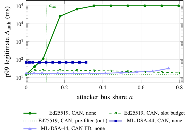
Fig. 5. Induced verification (Proposition 6), discrete-event simulation with verification CPU share \beta = 0.2 and the HCRL base load. Forged Ed25519 transfers cost the verifier 1.647 CPU-seconds per bus-second ( \rho_{\text{iv}} ). Beyond a_{\text{sat}} = 0.105 of the bus, the verification queue diverges and the legitimate signed stream is denied (values above 10^5 ms are clipped). ML-DSA-44 on classic CAN is immune, because its signature is too expensive to transmit for a flood to reach the CPU. On CAN FD the same scheme moves to \rho_{\text{iv}} = 0.226 .
