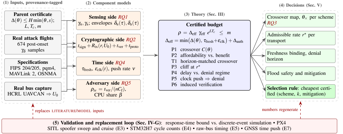
Fig. 1. Methodological framework. (1) Every input carries a provenance tag: measured on real flights or buses, derived, taken from a specification, or modelled. (2) Four component models quantify the two sides of the trade, sensing and cryptography, together with time and the flooding adversary. (3) The certified budget composes them into one inequality in metres, from which the propositions follow. (4) The decisions an engineer needs are read off the budget. (5) Simulation and hardware experiments replace modelled inputs with measured ones; because every number in the paper is generated from result files, a replacement propagates to the text automatically.
