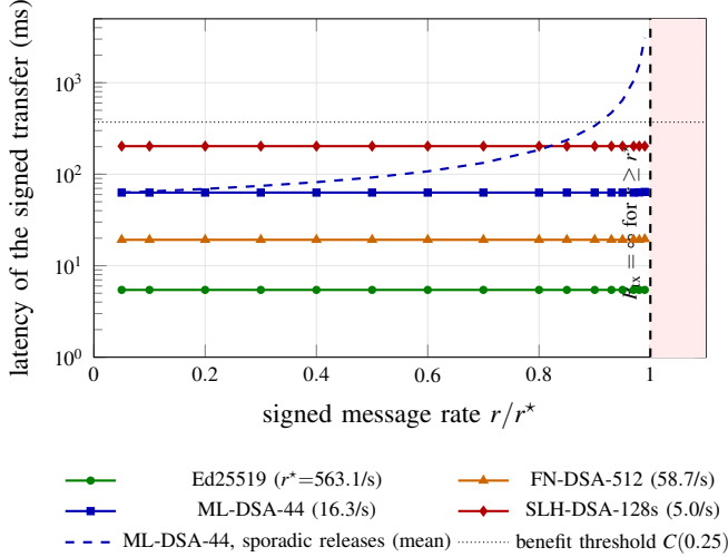
Fig. 3. The cost is a cliff, not a slope (Proposition 3). Solid lines show the busy-period bound of a signed transfer with periodic releases on classic CAN at 1 Mbit/s, above the base load U_0 = 0.099 derived from the HCRL UAVCAN capture. Below r^* the latency is essentially the transmission time of the signature; at r^* the busy period no longer closes, and the latency, and with it the certificate, is unbounded. With sporadic (Poisson) releases the cliff softens into a slope (dashed), which crosses the benefit threshold C(0.25) = 371 ms at r \approx 0.91 r^* .
