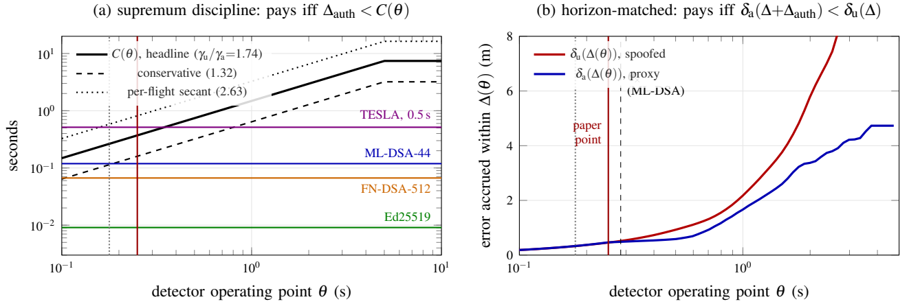
Fig. 4. The crossover map. (a) Under the supremum discipline of the parent certificate, one rate per configuration, the benefit threshold C(\theta) grows linearly in \theta until the slack saturates the hidden delay. Every per-message signature scheme that fits on the bus lies below the headline curve across the whole certified window. The vertical lines mark the benign floor (0.178 s) and the paper operating point (0.25 s). (b) Matching the horizon to the delay the detector actually admits changes the picture at tight settings. Within \Delta(0.25) = 0.5 s, the spoofed and the proxy estimator have accrued the same error to within 1 cm, so the data cannot show a benefit. On these envelopes, authentication pays from \theta_x = 0.284 s for ML-DSA-44 (Table V). Both panels use the jamming flight as a proxy for \gamma_a .
