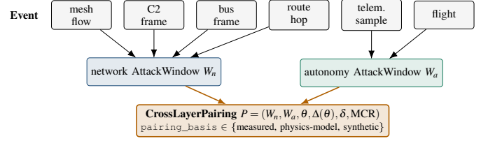
Fig. 2: Structure of the two-layer schema. Heterogeneous events from six datasets fold into typed network and autonomy AttackWindows ; a CrossLayerPairing joins one of each and records the detector operating point, the residual budget, the induced perturbation, and the mission outcome, tagged by how the coupling was established.
