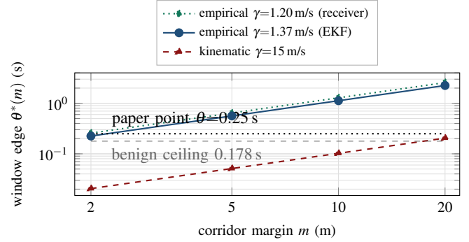
Fig. 8: The decisive sensitivity: the loosest detector setting \theta^*(m) = m/(\gamma e^{LT_c} H) whose worst-case evading tube still fits a corridor of margin m , per interface mapping. A mapping certifies the paper operating point iff its curve lies above the \theta=0.25 s line; the feasible region is bounded below by the measured benign residual ceiling (0.178 s, the FPR=0 floor). The measured rates clear the requirement \gamma_{\text{req}}=6.14 m/s at m=10 m by \sim 4.5\times ; the kinematic worst case fails at every margin.
