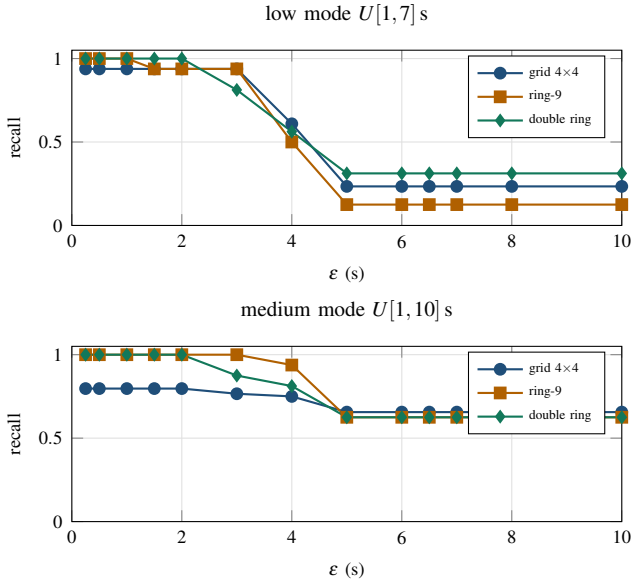
Fig. 3: The detector operating curve across all three topologies (grid, ring, double-ring), both delay regimes, 8 seeds \times 4 routing policies. Recall holds near its ceiling while \varepsilon stays under the 5 s contact-window slack, then falls onto a floor set by the missed-window self-exposure penalty (a delay past the slack costs a full TWiG period and is flagged at any \varepsilon ). False-positive rate is zero throughout; the measured benign residual ceiling is 0.178 s. The knee-and-floor shape is universal; the floor height is the topology-specific self-exposure probability.
