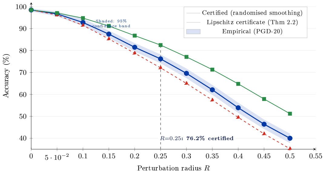
SDE-TGNN Certified Robustness vs Perturbation Radius R
