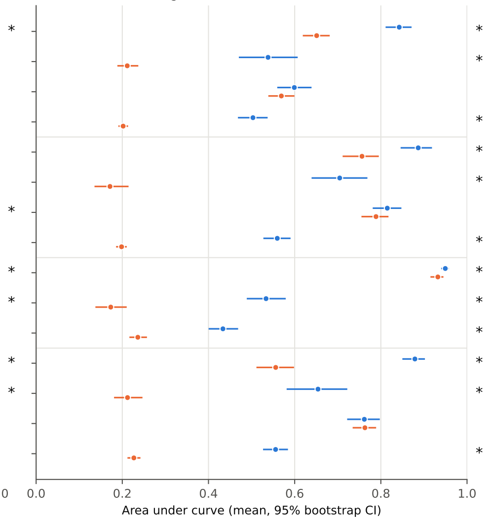
(b) Insertion AUC (higher = more faithful)
