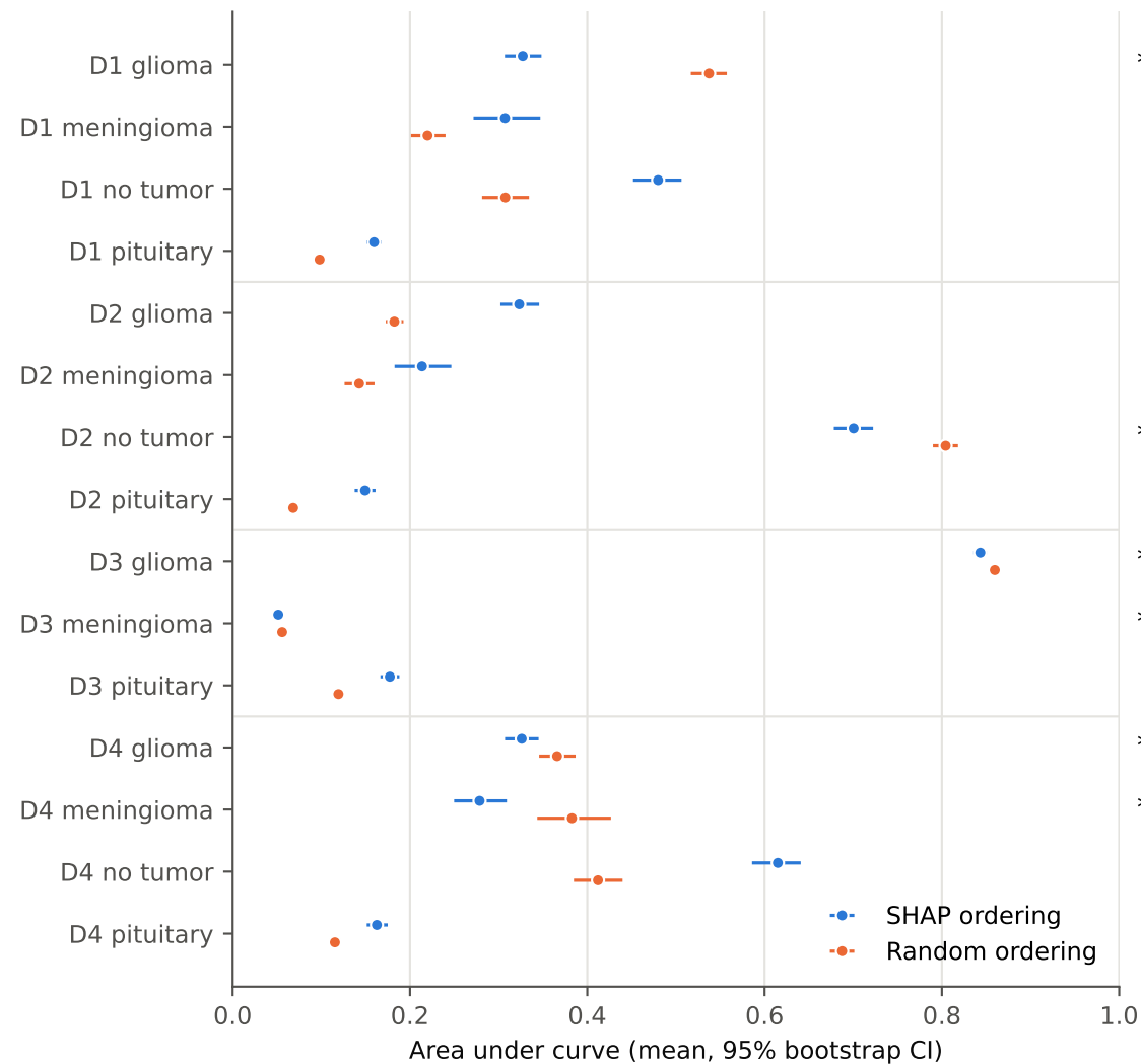
(a) Deletion AUC (lower = more faithful)
