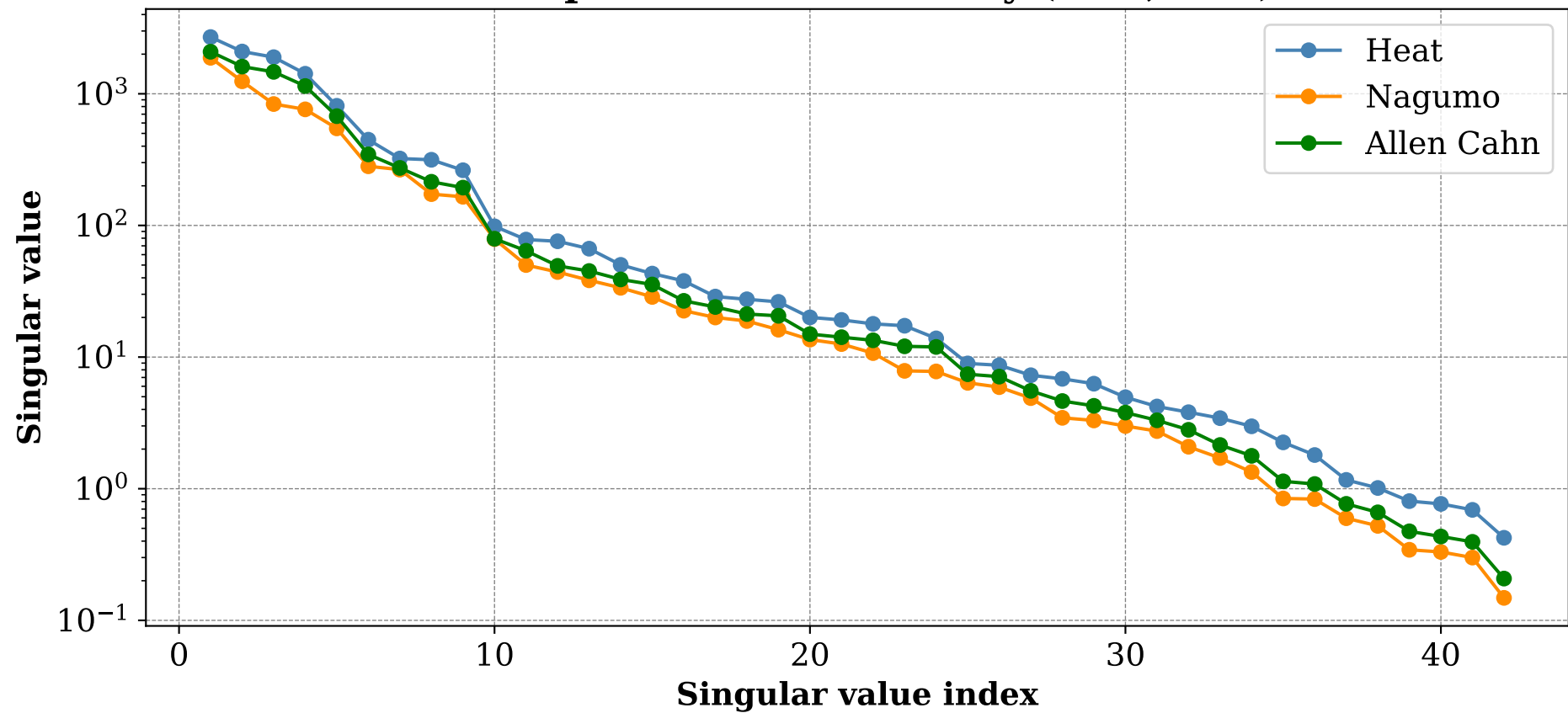
SVD spectrum of dictionary ( D=5 , P=6 )
