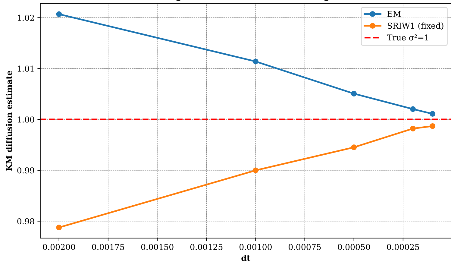
Convergence of KM estimate — nagumo
