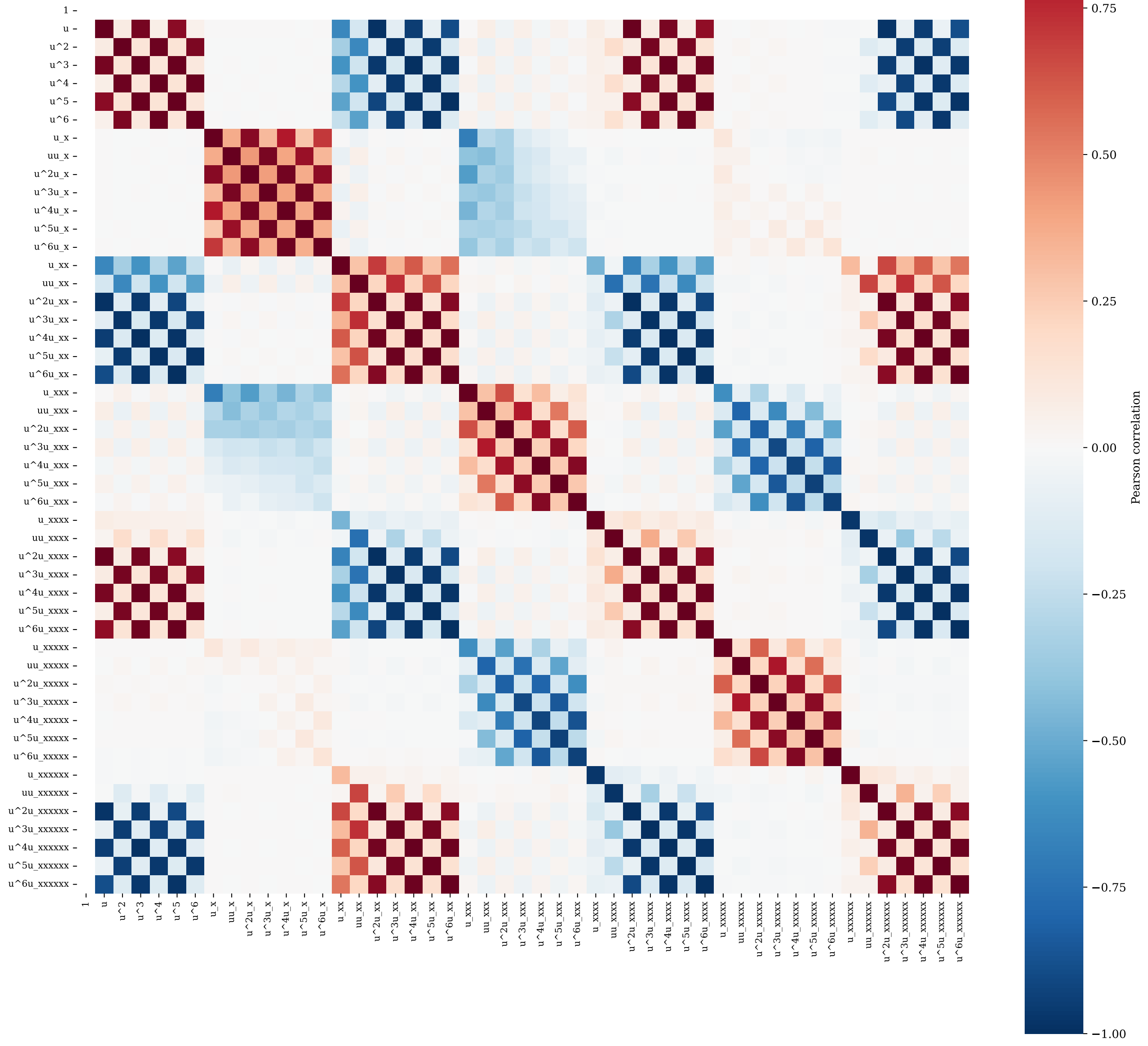
Dictionary correlation matrix - Allen_Cahn
