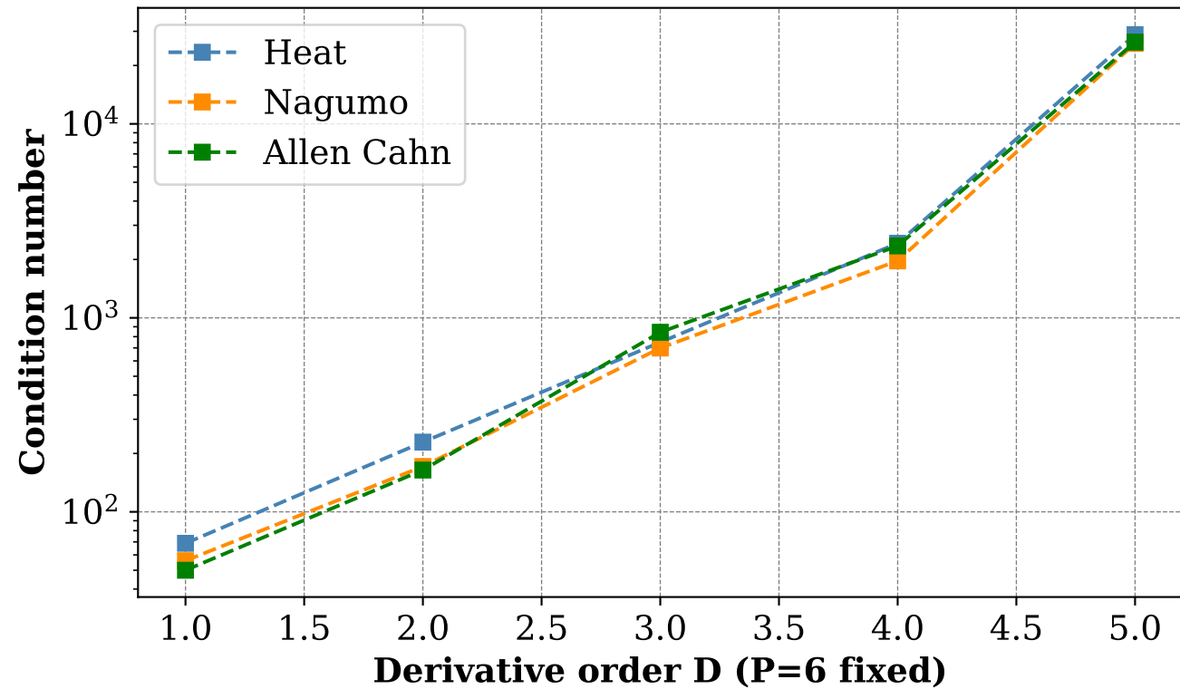
Condition number vs D
