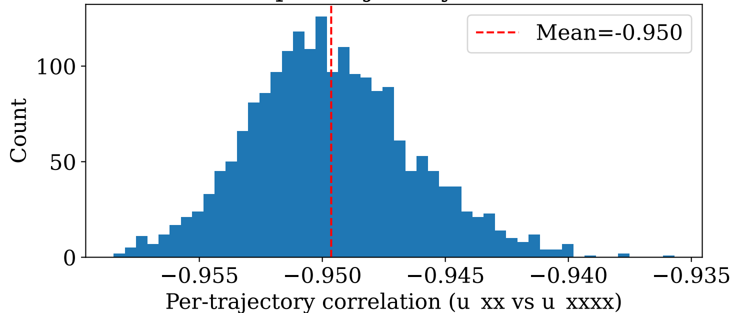
Distribution of per-trajectory correlations - Heat
