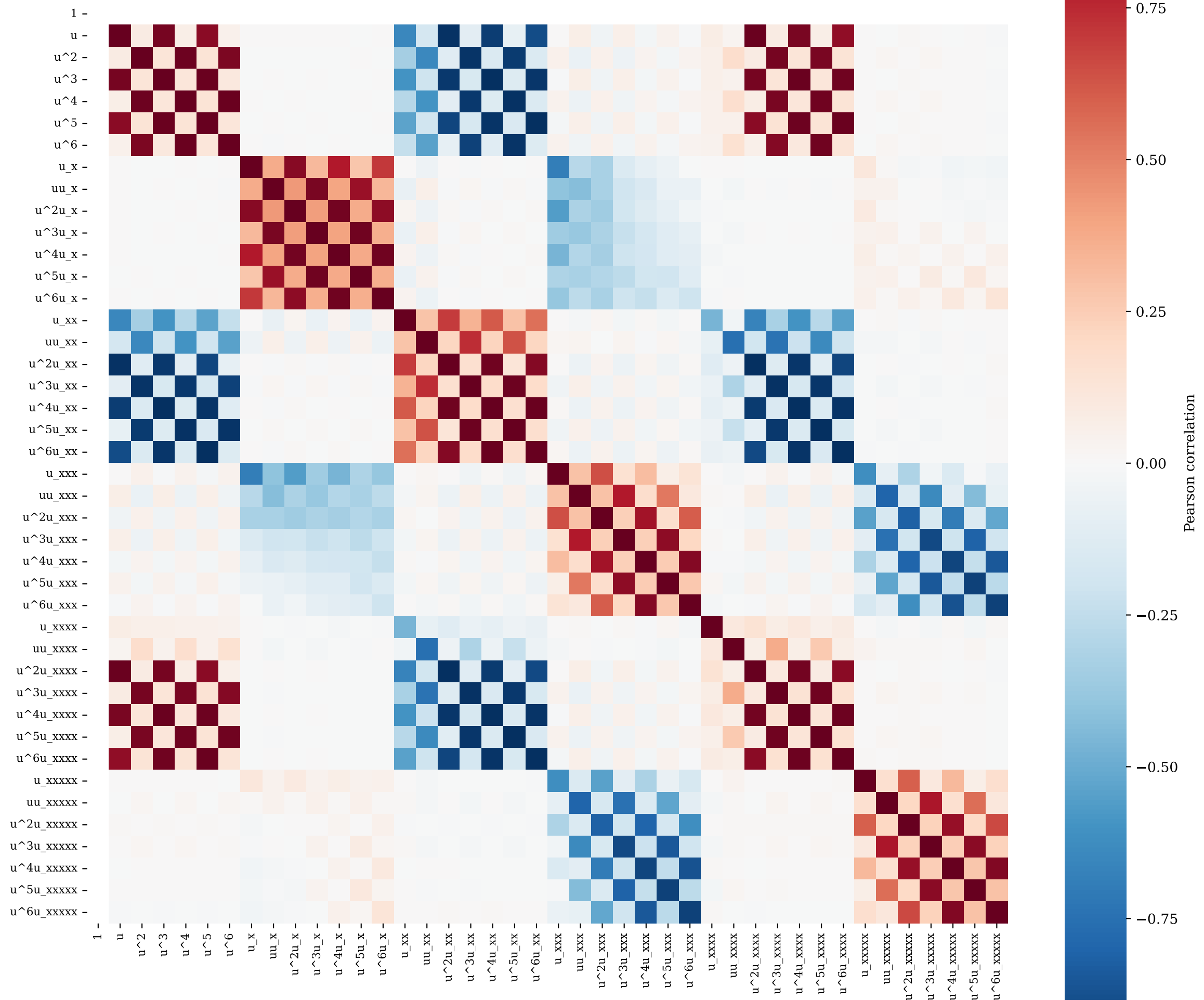
Dictionary correlation matrix - Allen_Cahn
