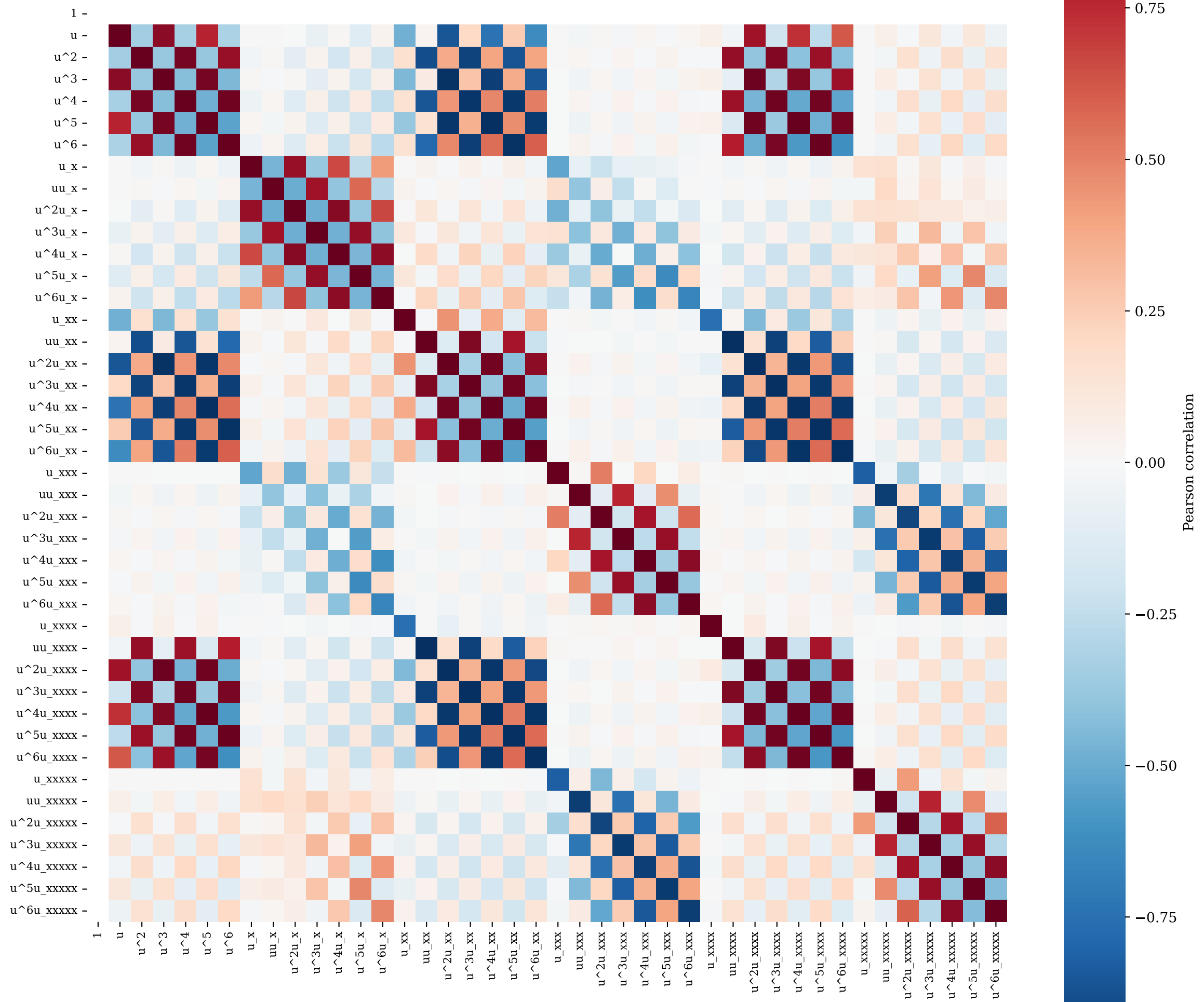
Dictionary correlation matrix - KdV
