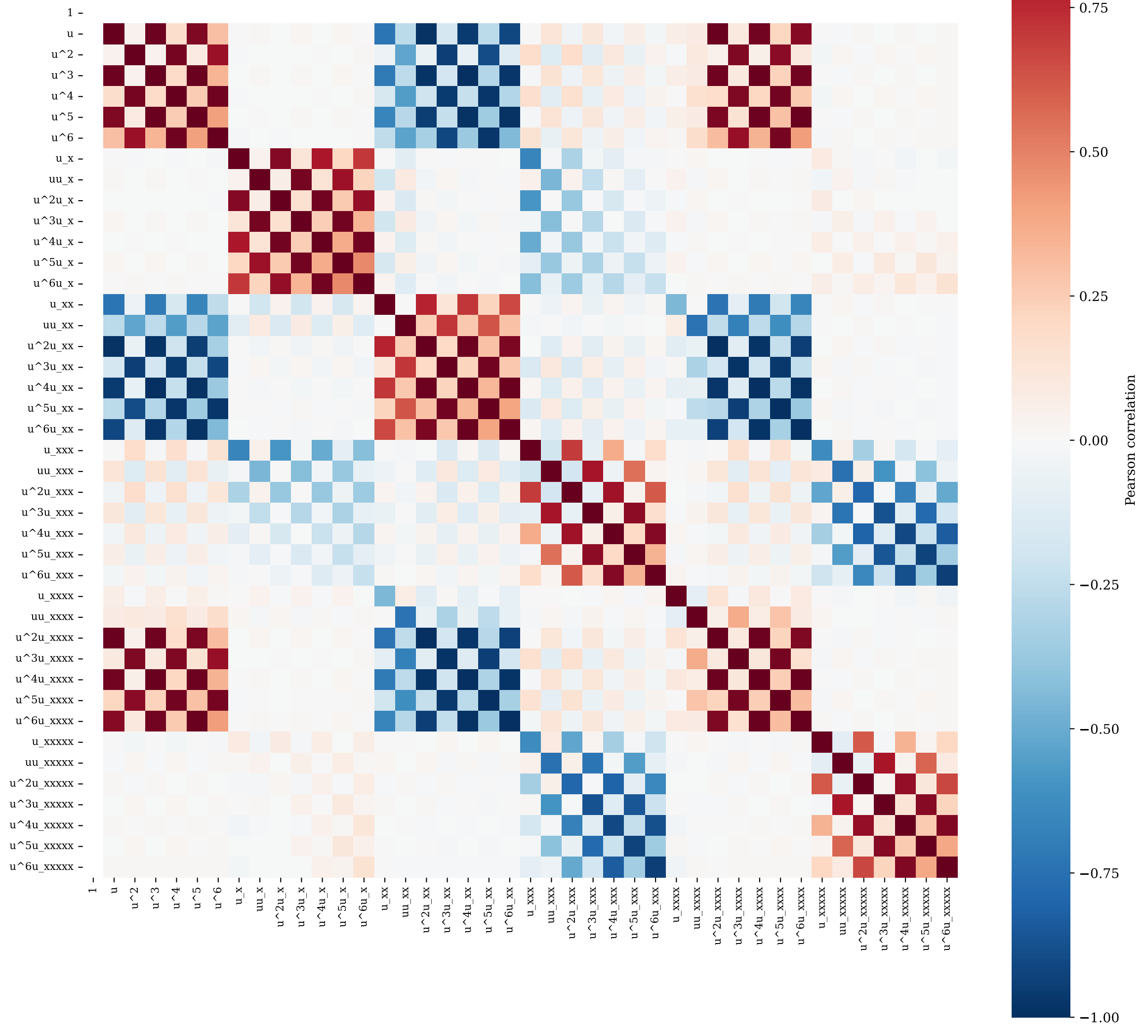
Dictionary correlation matrix - Nagumo
