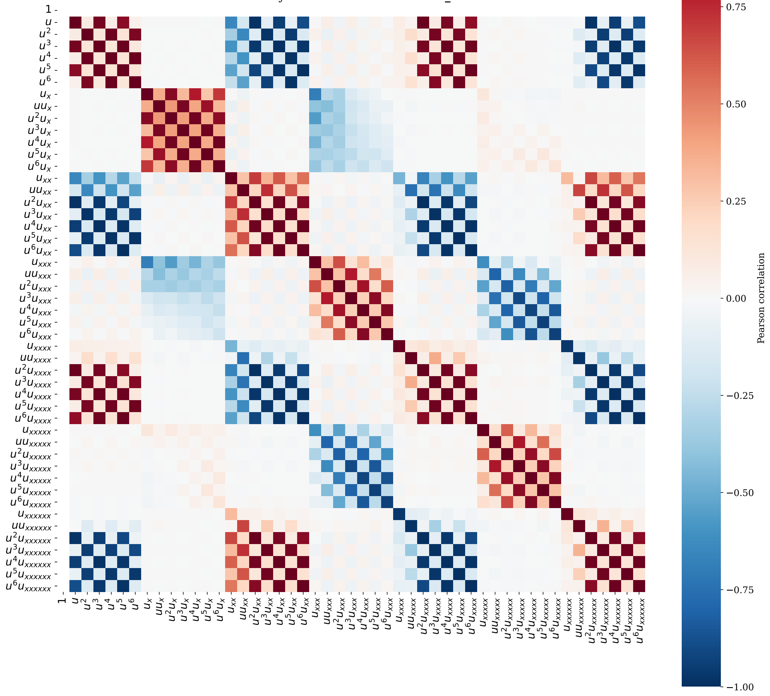
Dictionary correlation matrix - Allen_Cahn
