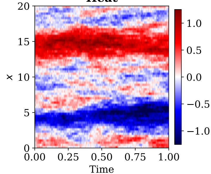
Heat
