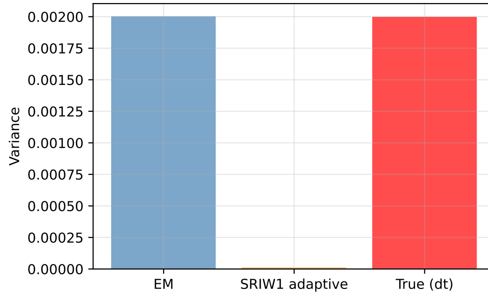
Increment variance (should be dt=0.002 )
