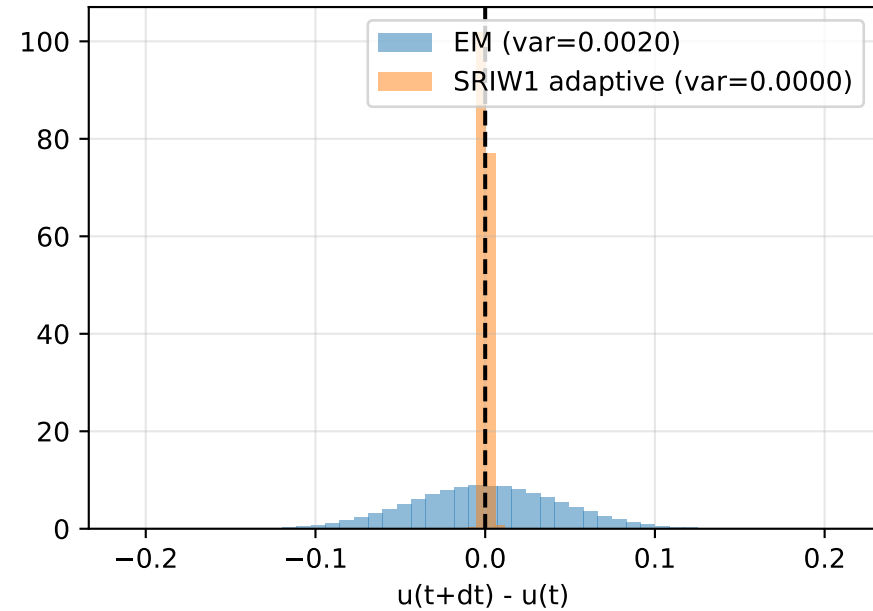
Increment distributions
