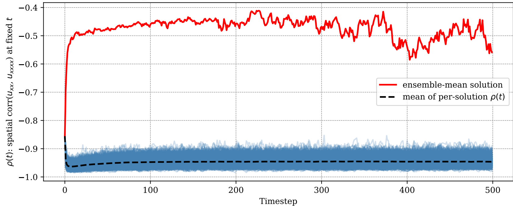
Allen_Cahn: per-timestep correlation, solutions vs. mean solution
