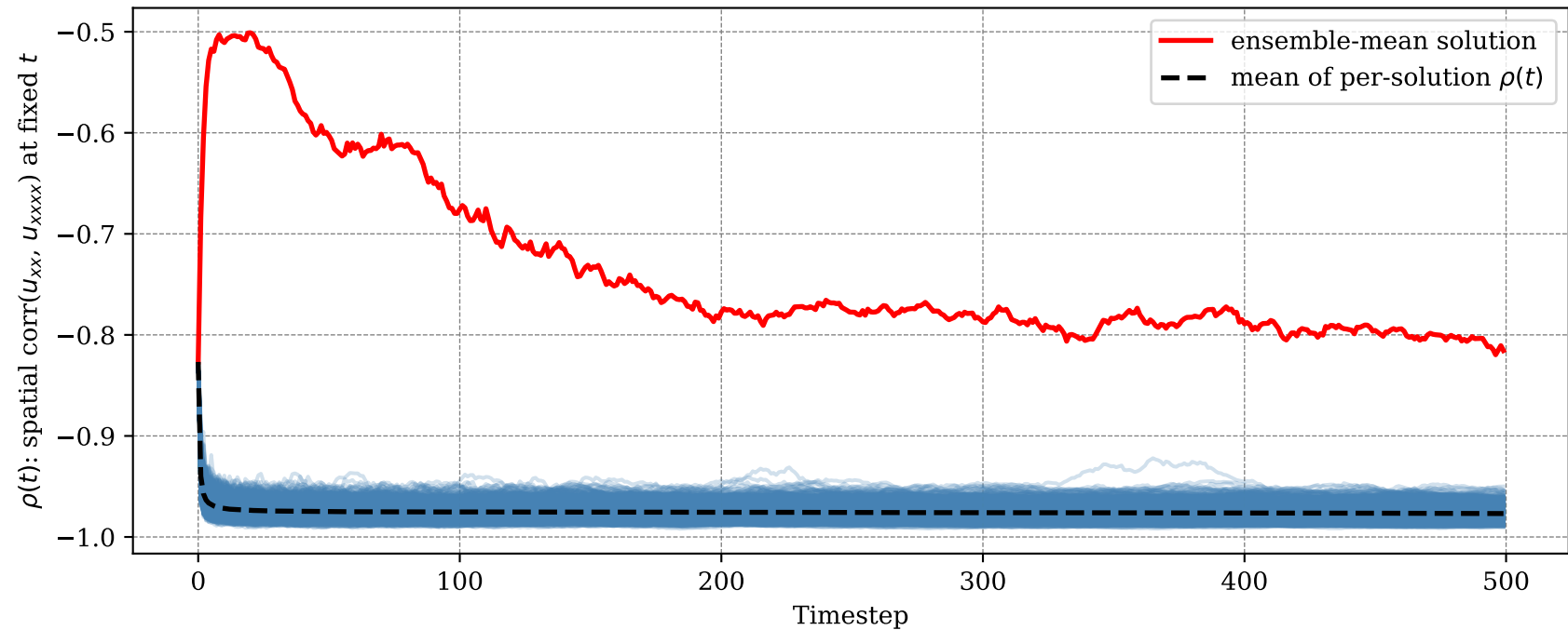
KdV: per-timestep correlation, solutions vs. mean solution
