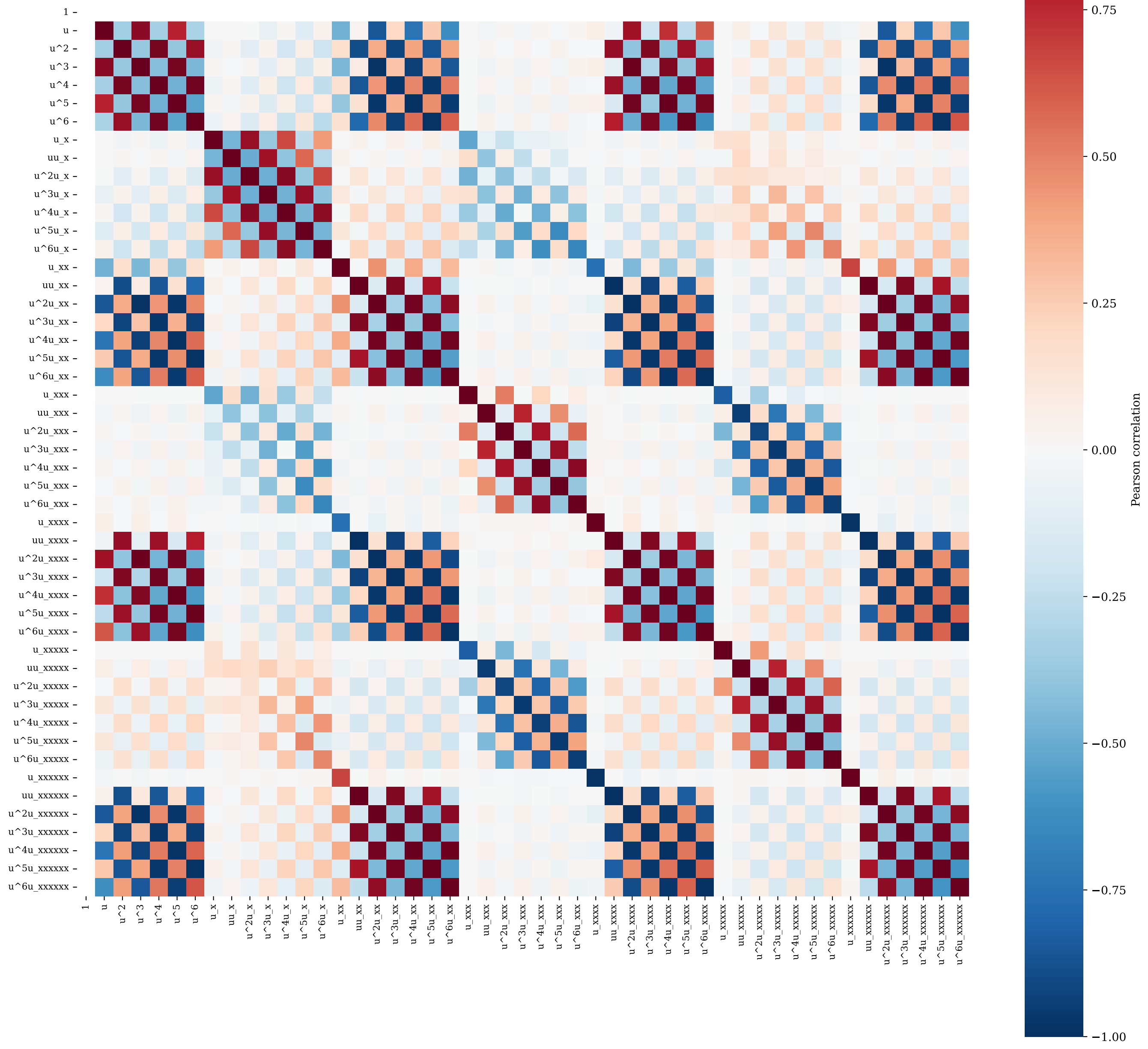
Dictionary correlation matrix - KdV
