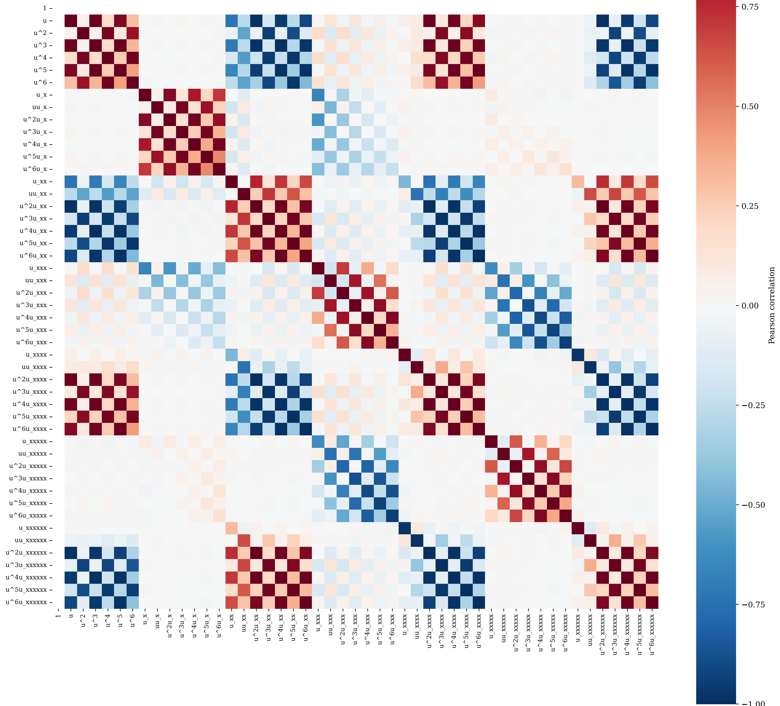
Dictionary correlation matrix - Nagumo
