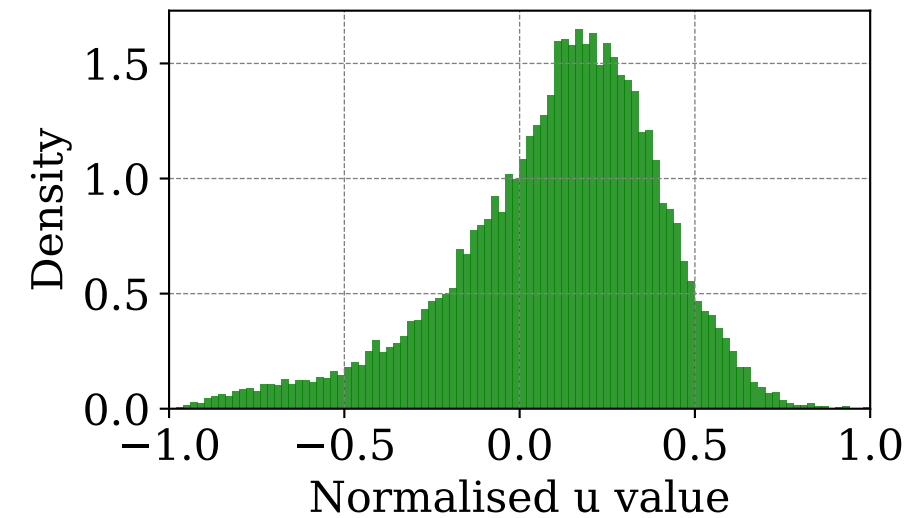
Allen Cahn
