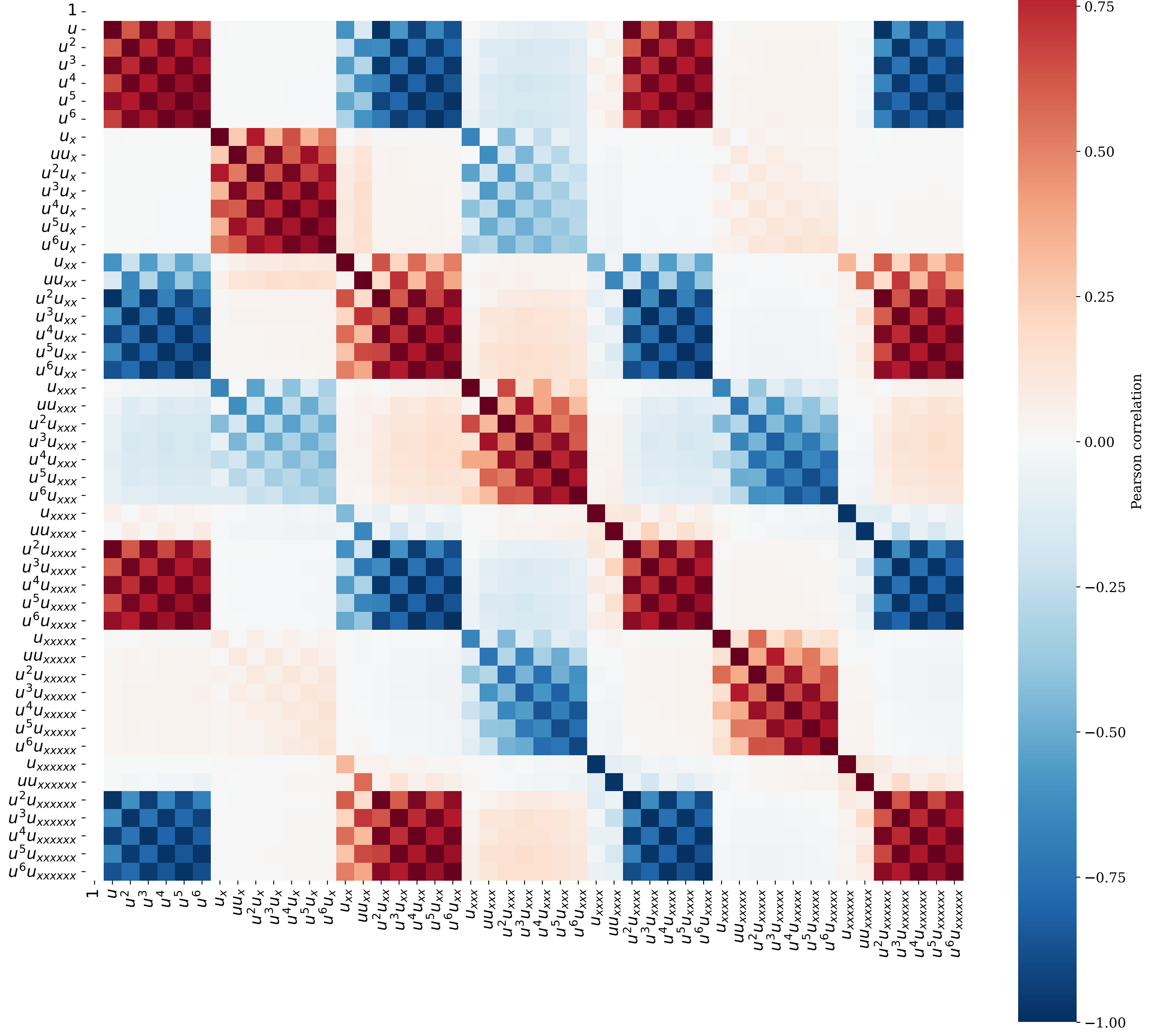
Dictionary correlation matrix - Heat
