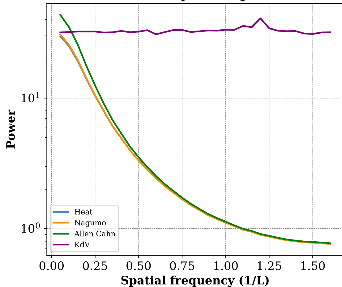
Fluctuation power spectrum
