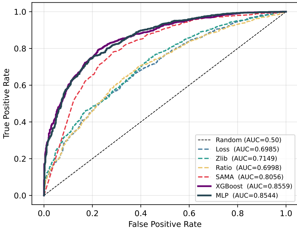
ROC Curves — Experiment 2
